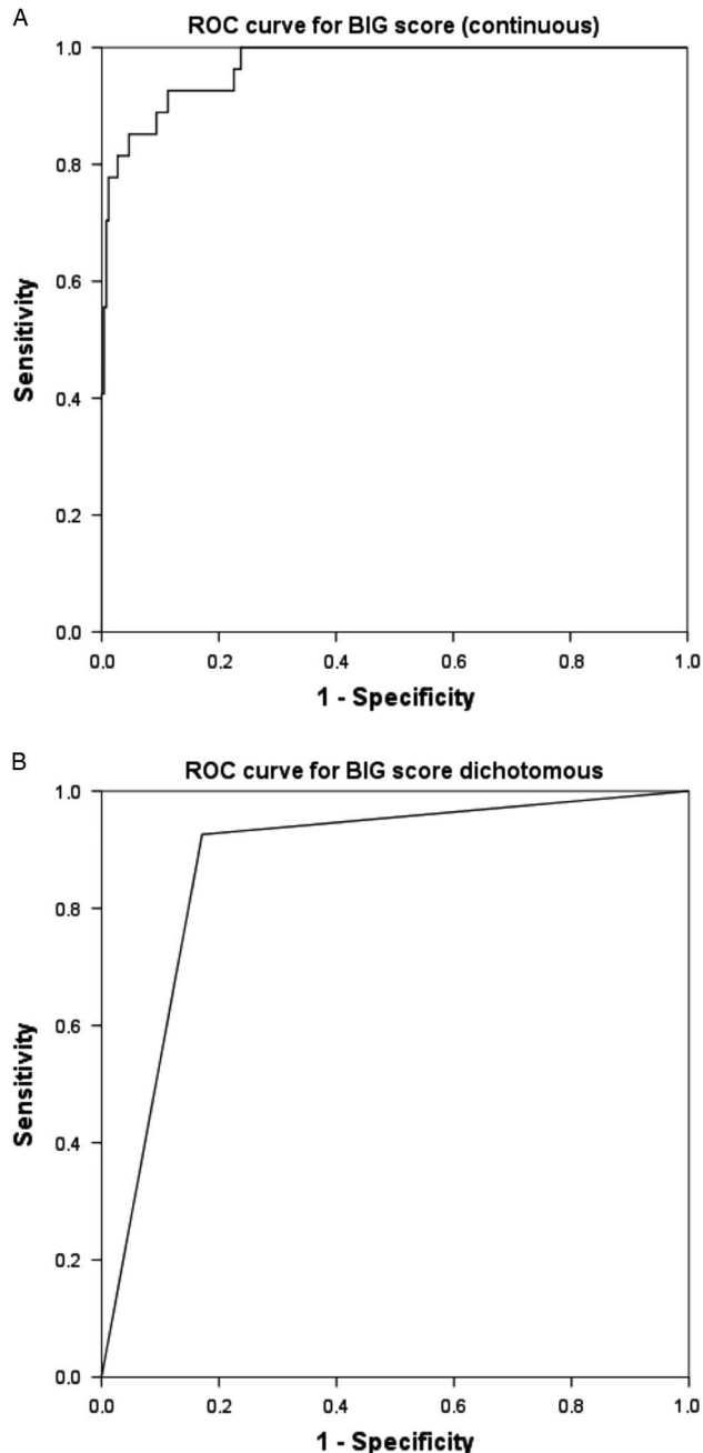
Figure 2. A) ROC curve for the BIG score (continuous) versus mortality. B) ROC curve for the BIG score (higher or lower than 16) versus mortality.
