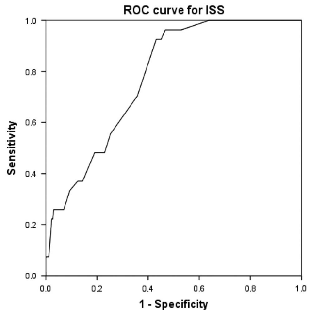
Figure 3. ROC curve for the ISS versus mortality.
