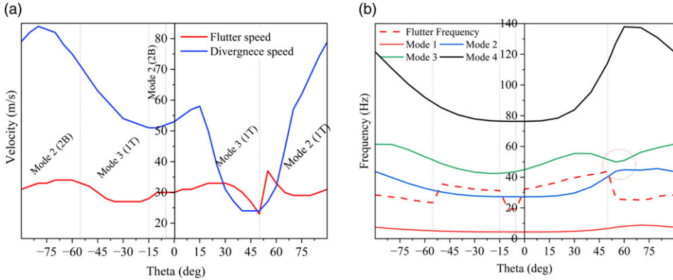
Figure 11. (a) Aeroelastic instability velocities vs theta (b) Flutter and the natural frequencies of the first four modes vs theta for 25° Aft swept composite plate.
