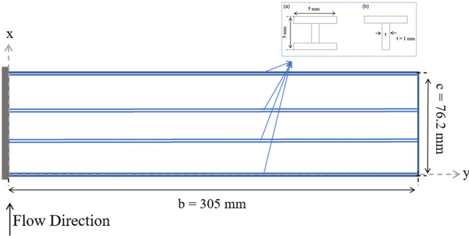
Figure 3. Unswept stiffened plate.
