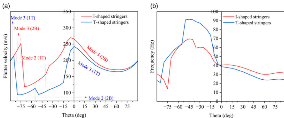
Figure 17. (a) Flutter speed vs theta (b) Flutter frequency vs theta for the unswept stiffened plate with 25° Aft swept I-shaped and T-shaped stringers.
