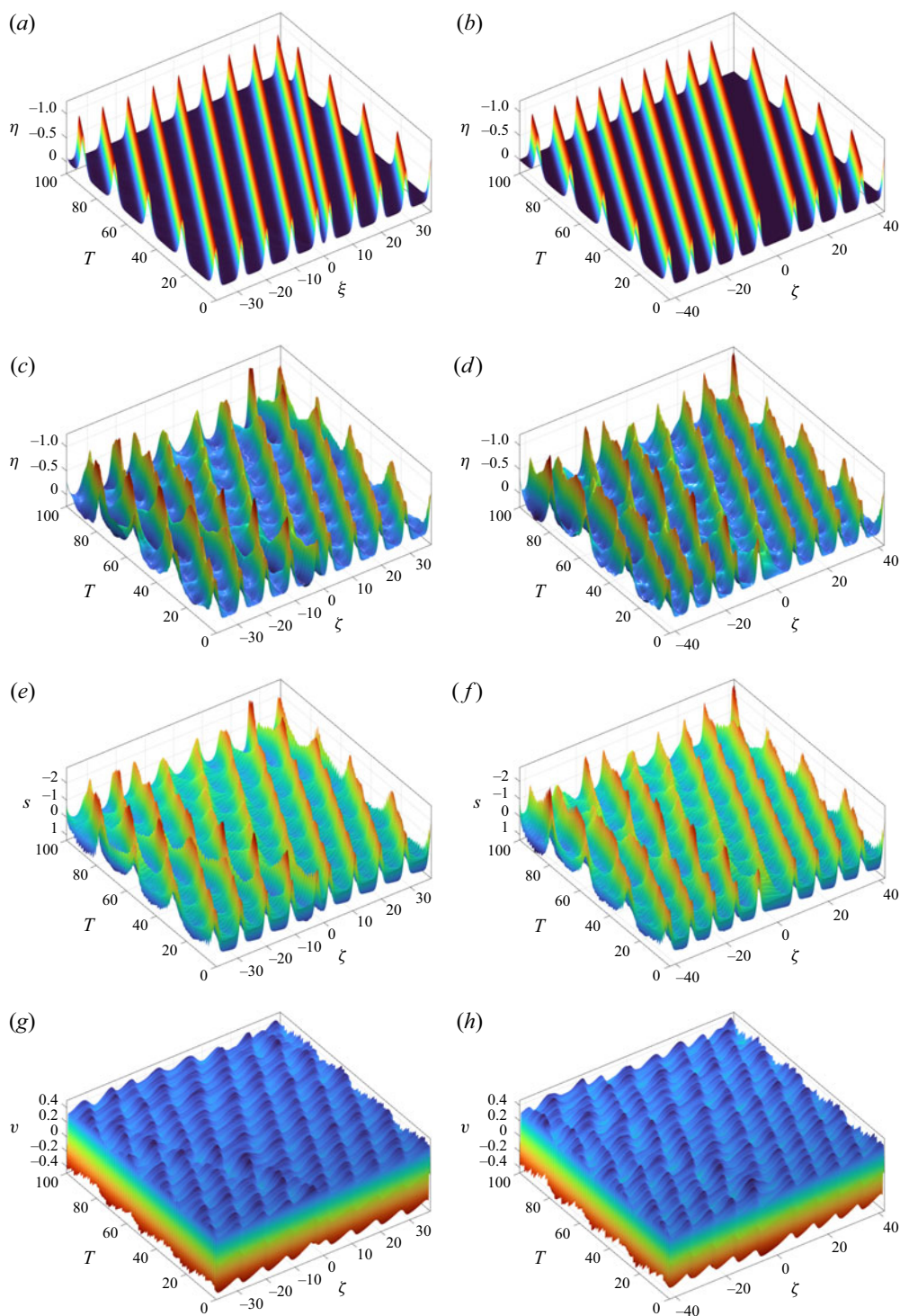
Figure 9. Numerical solution for a cnoidal wave with a contraction (a,c,e,g) and expansion (b,d,f,h) defect initial condition (view from below): (a,b) interfacial displacement in the absence of rotation, (c,d) interfacial displacement under the effect of rotation, (e,f) / (g,h) shear in the direction of wave propagation / orthogonal direction, under the effect of rotation.
