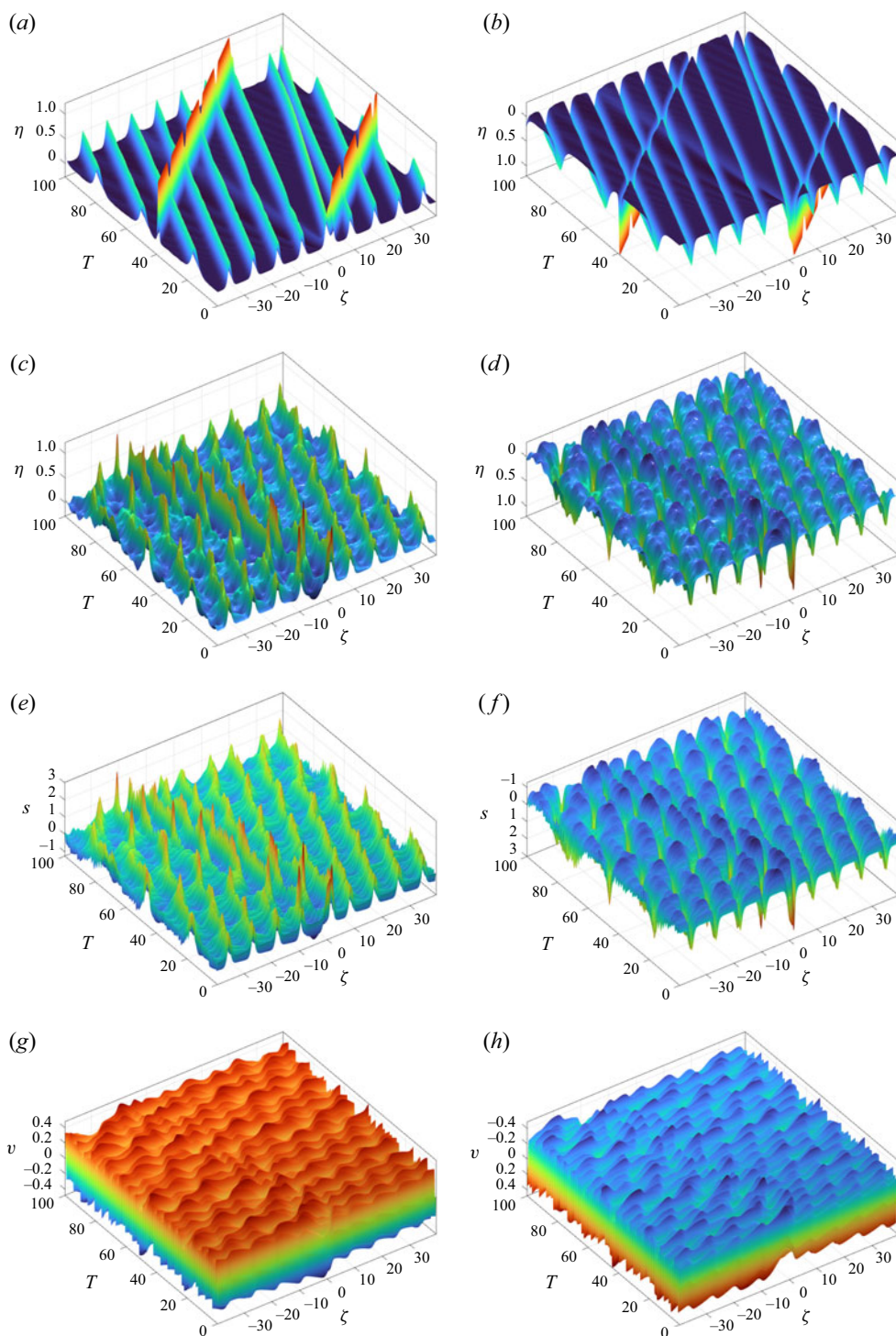
Figure 13. Numerical solution for a cnoidal wave with a generic localised defect initial condition (waves of elevation, view from above ( a,c,e,g ) and below ( b,d,f,h )): ( a,b ) interfacial displacement in the absence of rotation, ( c,d ) interfacial displacement under the effect of rotation, ( e,f ) / ( g,h ) shear in the direction of wave propagation / orthogonal direction, under the effect of rotation.
