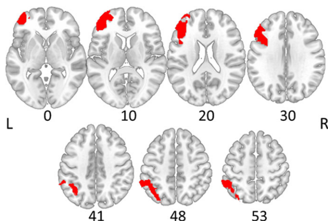
Lateral components of the fronto-parietal network according to Yeo functional connectivity atlas
