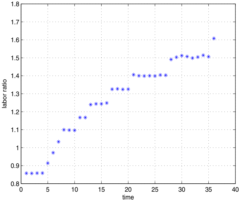
Figure 3. Evolution of \psi_t . The stars represent \psi at each period of the time interval explored with simulations.
