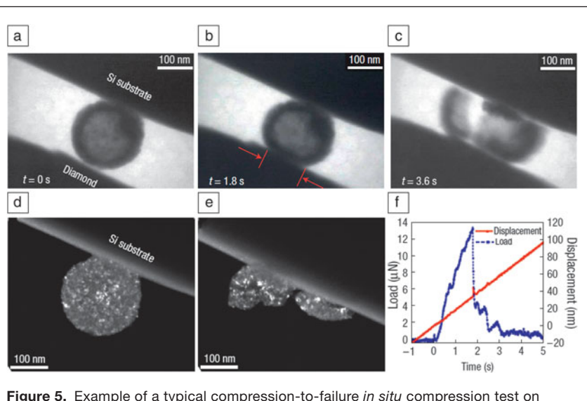
Figure 5. Example of a typical compression-to-failure in situ compression test on an individual nanocrystalline hollow CdS sphere. (a–c) Extracted video frames of the in situ compression test, corresponding to time t = (a) 0 s, (b) 1.8 s, and (c) 3.6 s. The estimated contact diameter is shown in red in (b). (d–e) Dark-field transmission electron microscope images of the hollow nanocrystalline CdS ball resting on the Si substrate (d) before and (e) after the compression test. (f) Load and displacement data from the loading portion of the in situ test versus time. The experiment was run under displacement control. Reproduced with permission from Reference 15. © 2008 Nature Publishing Group.
