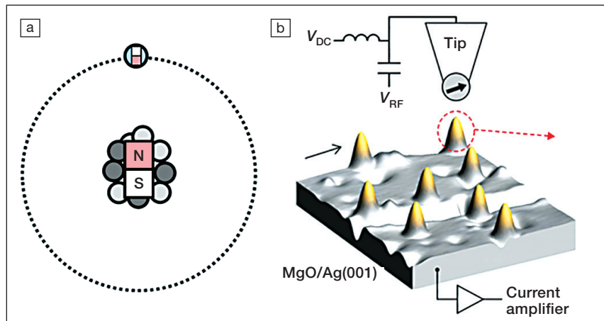
(a) The nucleus of an atom acting as a magnet, with the magnet of the electron pointing in the opposite direction. (b) A scanning tunneling microscope tip interacts with a Cu atom on a surface. Credit: Nature Nanotechnology .
