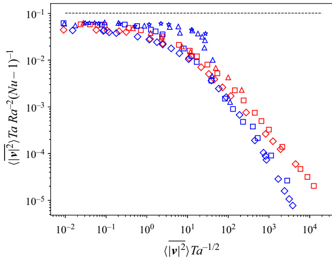
Figure 5. Value of \langle |\mathbf{v}|^2 \rangle Ta Ra^{-2} (Nu - 1)^{-1} as a function of \langle |\mathbf{v}|^2 \rangle Ta^{-1/2} for Pr = 7 (red symbols) and Pr = 0.7 (blue symbols). The symbol shape stands for Ta = 10^4 (diamonds), 10^6 (squares), 10^8 (triangles) and 10^{10} (stars). The dashed horizontal line indicates 1/\pi^2 .
