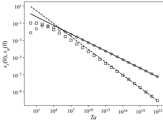
Figure 3. Values of s_\varphi(0) (circles) and s_s(0) (squares) together with the functions 1.23Ta^{-1/3} (solid) and 9Ta^{-1/2} (dashed).
