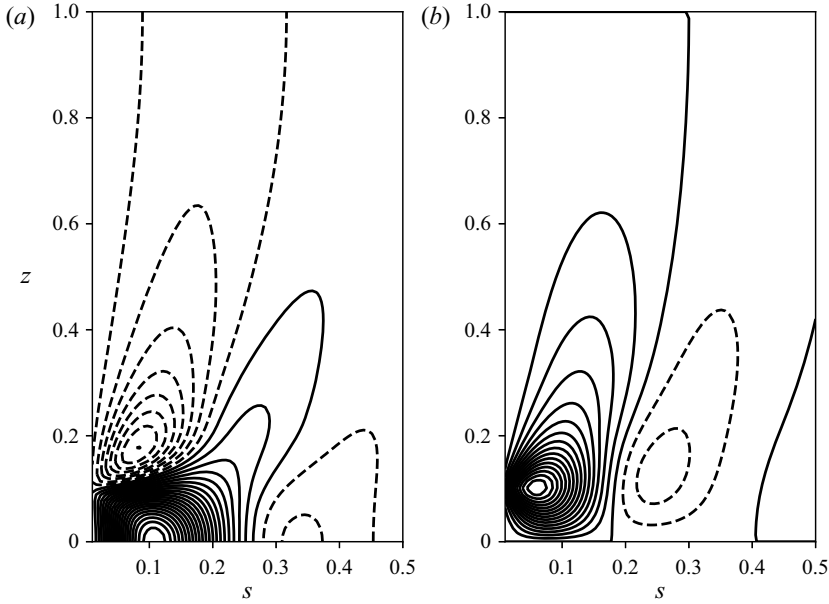
Figure 4. Contour plot of the circulation sv_{G,\phi} (a) and the streamlines of the meridional part of \mathbf{v}_G , (v_{G,s}, 0, v_{G,z}) (b) in a vertical plane for a source located at height z = 0.1 on the axis s = 0 for Ta = 10^6 . Dashed contour lines indicate anticyclonic circulation.
