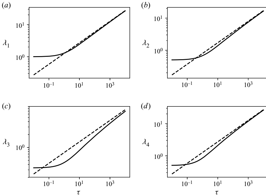
Figure 1. The largest root of the polynomials in (3.15) (a), (3.29) (b), (3.34) (c) and (4.18) (d) as a function of \tau together with the asymptotic dependences (2\tau)^{1/3} (a), (\tau/2)^{1/3} (b), (\tau/3)^{1/4} (c) and (2\tau)^{1/3} (d) shown with dashed lines.
