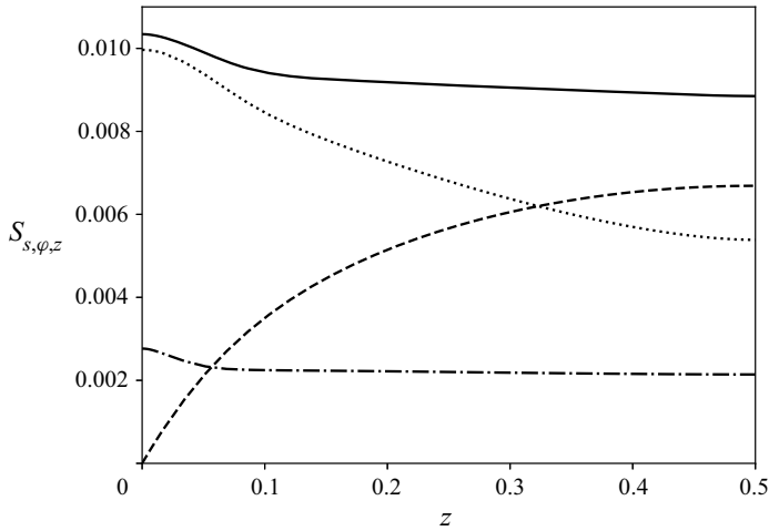
Figure 2. Values of s_s (dot dashed), s_\varphi (dotted) and s_z (dashed) as functions of height z for Ta = 10^6 . The solid line shows \sqrt{s_s^2 + s_\varphi^2 + s_z^2} .
