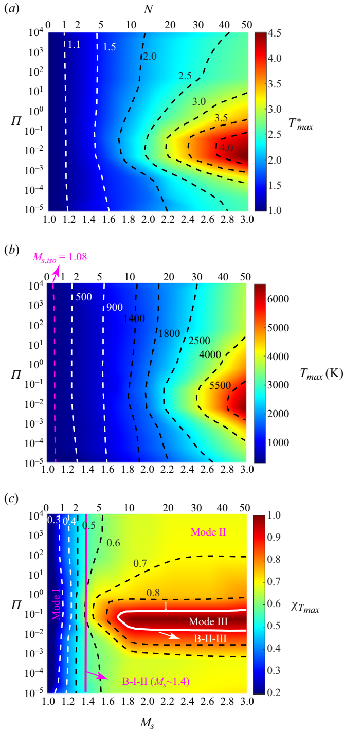
Figure 15. Contour maps of T_{max}^* (a), T_{max} (b) and \chi T_{max}^* (c) in the parameter space ( M_s , \Pi ). Three distinct heating modes, mode I: the gas-filtration-dominated mode, mode II: the rear-surface-dominated mode and mode III: persistent heating mode, are delineated by two boundaries. Boundaries between different modes are represented by the pink and white solid lines which are denoted as B-I-II and B-II-III, respectively.
