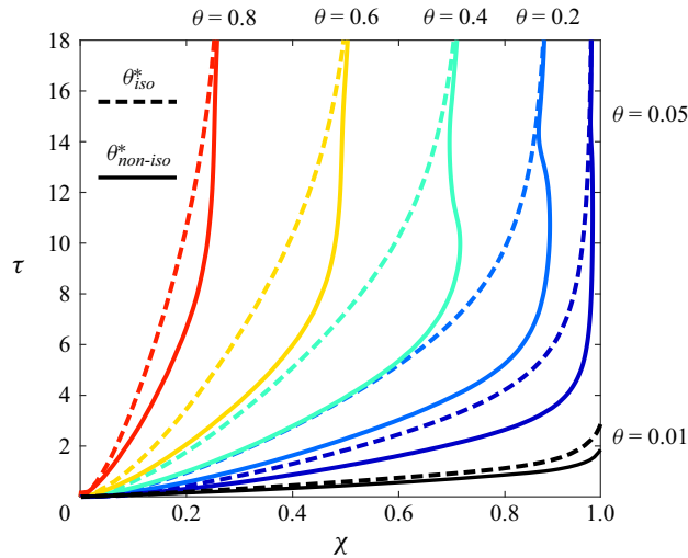
Figure 7. Temporospacial evolutions of the isothermal and non-isothermal diffusing pressure fields in C-1.43-50. Dashed and solid curves represent the isolines of \theta_{iso}^*(\chi, \tau) and \theta_{non-iso}^*(\chi, \tau) , respectively.
