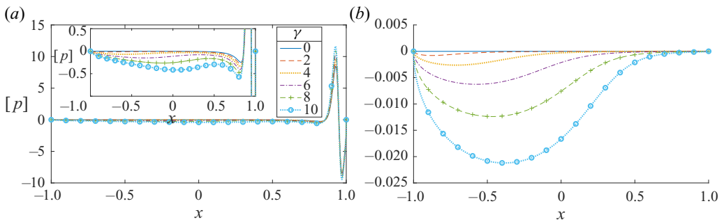
FIGURE 19. Effect of varying \gamma on the jump in surface pressure, [p] , for k_0 = 0.5 . (a) Shows the real part of [p] , (b) the imaginary part. In all cases the porosity at the trailing edge is fixed at \alpha_T = 0.3 , and at the leading edge at \alpha_L = 0 .
