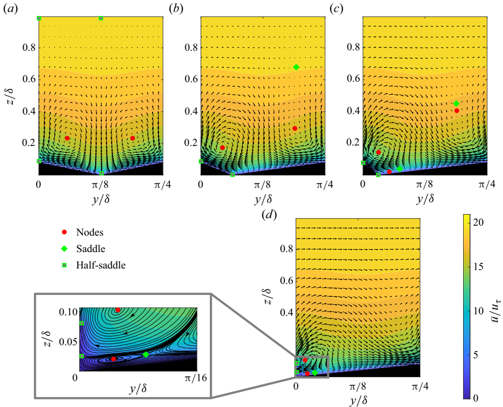
Figure 2. Contours of the phase-averaged mean streamwise velocity with superimposed in-plane velocity vectors (downsampled for clarity): (a) R1, (b) R3, (c) R7, (d) R\infty . Locations of critical points in the flow are marked in each panel. For critical points located at the spanwise boundaries only one point is shown.
