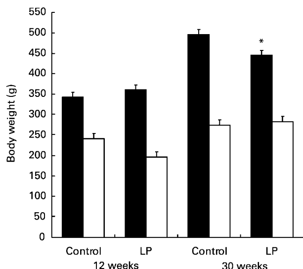
Fig. 4. Body weights of offspring at 12 and 30 weeks of age. ■, Male, □, female. For details of foods and procedures, see Table 1 and p. 514. At 12 weeks: low-protein (LP)-exposed female rats n = 5 , control female rats n = 9 , LP-exposed male rats n = 6 , control male rats n = 11 . At 30 weeks: LP-exposed female rats n = 5 , control female rats n = 5 , LP-exposed male rats n = 6 , control male rats n = 12 . There were significant effects (three-way ANOVA) of age ( P < 0.001 ), gender ( P < 0.001 ) and age \times gender \times maternal diet ( P = 0.017 ) on weight. Mean value was significantly different from that of control rats of the same age: * P < 0.05 .
