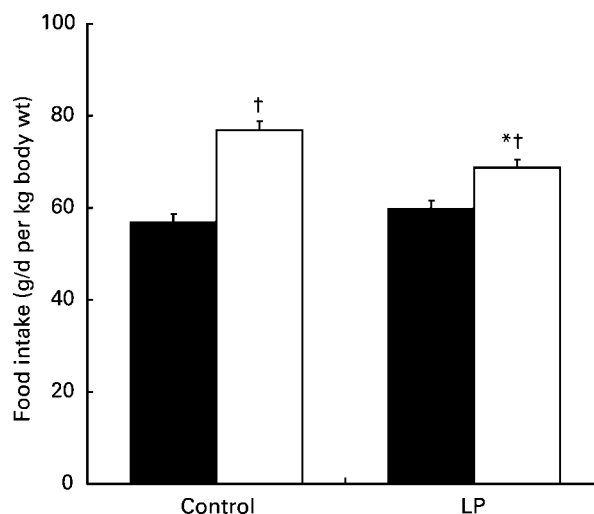
Fig. 1. Intake of standard laboratory chow diet by 12-week-old rats. ■, Male; □, female. For details of procedures, see p. 514. Values are means with their standard errors shown by vertical bars (low-protein (LP)-exposed female rats n 5, control female rats n 7, LP-exposed male rats n 6, control male rats n 12). There were significant effects (two-way ANOVA) of gender ( P < 0.001 ) and gender \times maternal diet ( P = 0.001 ). Mean value was significantly different from that of the control group of the same gender: * P < 0.05 . Mean values were significantly different from those of male rats in the same dietary group: † P < 0.05 .
