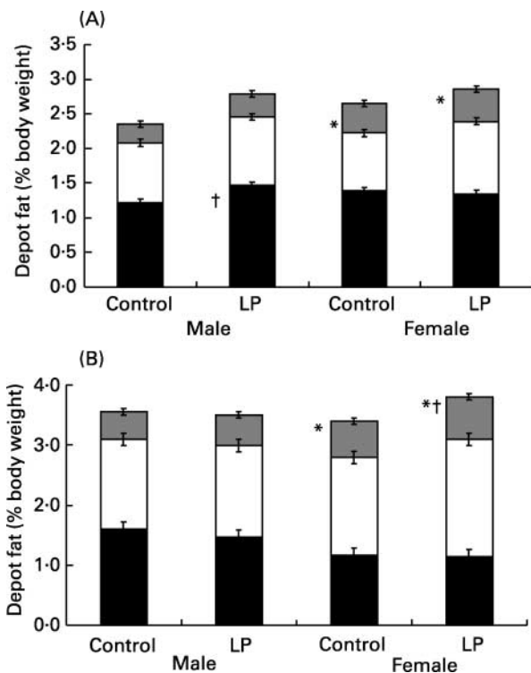
Fig. 5. Size of discrete adipose tissue depots. For details of foods and procedures, see Table 1 and p. 514. ■, Gonadal; □, perirenal, ■, intrascapular. (A), 12 weeks of age: values are means with their standard errors shown by vertical bars (LP-exposed female rats n 5, control female rats n 9, LP-exposed male rats n 6, control male rats n 11). There were significant effects (two-way ANOVA) on gonadal fat depot size in male rats of maternal diet ( P=0.01 ) and on the white adipose component of the intrascapular depot by gender ( P=0.007 ). Mean values were significantly different from those of male rats in the same maternal diet group: * P<0.05 . Mean value was significantly different from that of male control rats: † P<0.05 . (B), 30 weeks of age: values are means with their standard errors shown by vertical bars (LP-exposed female rats n 5, control female rats n 7, LP-exposed male rats n 6, control male rats n 12). There were significant effects (two-way ANOVA) on the brown adipose tissue component of the intrascapular depot of gender ( P=0.002 ) and maternal diet ( P=0.027 ). Mean values were significantly different from those of male rats in the same maternal diet group: * P<0.05 . Mean value was significantly different from that of male control rats: † P<0.05 .
