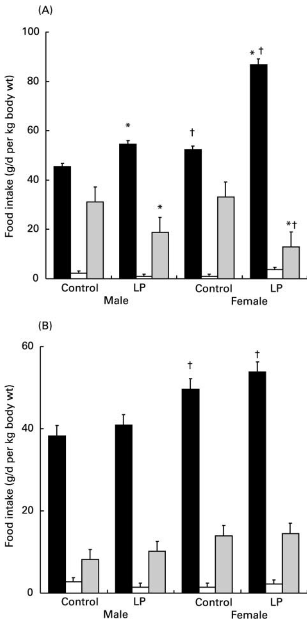
Fig. 2. Self-selection of high-fat, high-carbohydrate and high-protein foods by rats exposed to control or low-protein (LP) diets in utero . ■, Fat; □, protein; ■, carbohydrate. For details of foods and procedures, see Table 1 and p. 514. (A), 12-week-old rats: values are means with their standard errors shown by vertical bars (LP-exposed female rats n 5, control female rats n 9, LP-exposed male rats n 6, control male rats n 11). There were significant effects (two-way ANOVA) of maternal diet ( P=0.001 ), gender ( P=0.002 ) and gender \times maternal diet ( P=0.045 ) on consumption of the high-fat food. There was a significant effect of maternal diet on consumption of high-carbohydrate food ( P=0.013 ). Mean values were significantly different from control rats of the same gender: * P<0.05 . Mean values were significantly different from male rats within the same maternal dietary group: † P<0.05 . (B), 30-week-old rats: values are means with their standard errors shown by vertical bars (LP-exposed female rats n 5, control female rats n 7, LP-exposed male rats n 6, control male rats n 12). There were significant effects (two-way ANOVA) of gender on consumption of high-fat food ( P=0.002 ). Mean values were significantly different from those of male rats within the same maternal dietary group: † P<0.05 .
