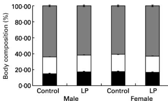
Fig. 6. Whole carcass composition at 12 weeks of age. For details of foods and procedures, see Table 1 and p. 514. ■, Fat; □, protein; ■, water. Values are means with their standard errors shown by vertical bars (LP-exposed female rats n 5, control female rats n 9, LP-exposed male rats n 6, control male rats n 11). There were no significant effects of maternal diet or gender.
