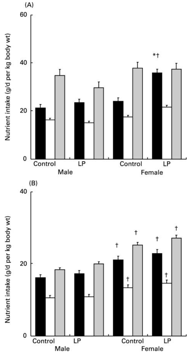
Fig. 3. Macronutrient intakes of rats exposed to control or low-protein (LP) diets in utero and allowed to self-select foods. ■, Fat; □, protein; ■, carbohydrate. For details of foods and procedures, see Table 1 and p. 514. (A), 12-week-old rats: values are means with their standard errors shown by vertical bars (LP-exposed female rats n 5, control female rats n 9, LP-exposed male rats n 6, control male rats n 11). There were significant effects (two-way ANOVA) of maternal diet ( P=0.002 ), gender ( P=0.001 ) and gender \times maternal diet ( P=0.023 ) on consumption of fat. There was a significant effect of gender on consumption of protein ( P<0.001 ). Mean value was significantly different from that of control rats of the same gender: * P<0.05 . Mean value was significantly different from that of male rats within the same maternal dietary group: † P<0.05 . (B), 30-week-old rats: values are means with their standard errors shown by vertical bars (LP-exposed female rats n 5, control female rats n 7, LP-exposed male rats n 6, control male rats n 12). There were significant effects (two-way ANOVA) of gender on intakes of fat ( P<0.001 ), carbohydrate ( P<0.001 ) and protein ( P<0.001 ). Mean values were significantly different from those of male rats within the same maternal dietary group: † P<0.05 .
