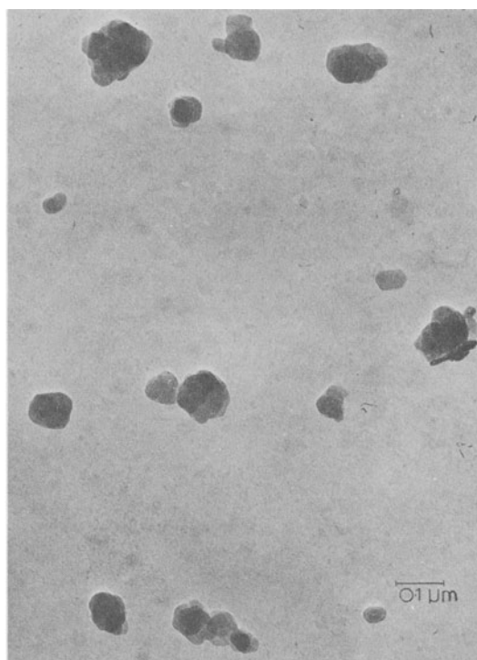
Fig. 5. Sample of sodium illite (Muloorina) dispersed onto a Cytochrome C film from an upright drop.
