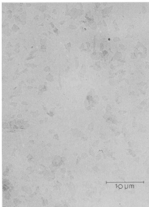
Fig. 3. Fine fraction of Na-montmorillonite (Wyoming) dispersed onto a Cytochrome C film from an upright drop.
