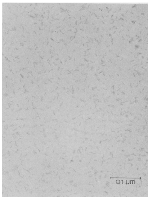
Fig. 1. Polycations in a solution of 0.1 M \text{FeCl}_3 with \text{OH}/\text{Fe} = 2.0 aged for 28 days at 20^\circ\text{C} . Close examination shows the rods to be made up of dot-like material similar to that shown in Fig. 2.
