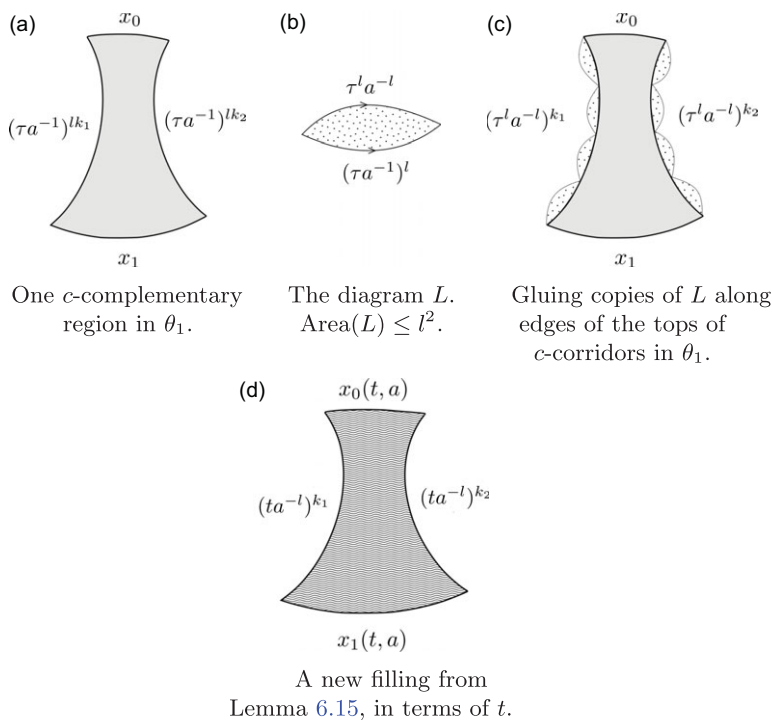
Figure 21. Converting a c -complementary region filling from \theta_1 over Q_1^c to one for \theta_l over Q_l .
