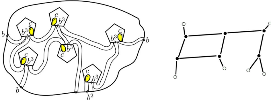
Figure 6. From capping faces and partial corridors in \overline{\Delta} , construct a graph \Gamma . Black vertices correspond to capping faces, white vertices correspond to 1-cells labeled b in \partial\overline{\Delta} , and the edges correspond to partial b -corridor.
