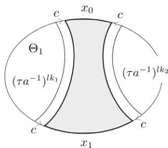
Figure 20. The quadratic area diagram \theta_1 .
