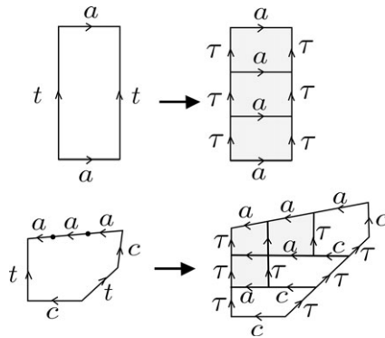
Figure 16. Converting \theta_0 from Q_l to Q_l^\tau (illustrated with l = 3 ).
