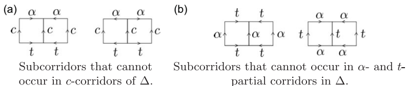
Figure 14. Non-reduced subcorridors not occurring in \Delta .
