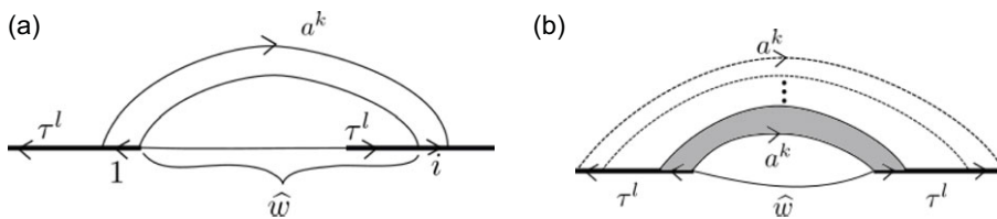
A \tau in position 1 in a \tau -segment can only pair with another initial \tau .
