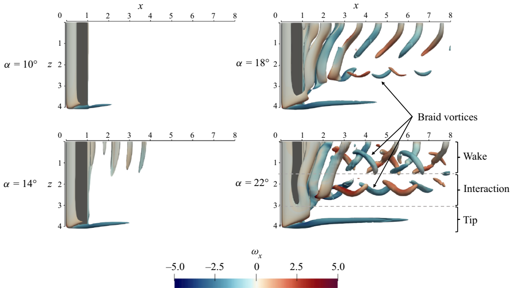
Figure 5. Effect of \alpha on instantaneous DNS solution shown with isocontours of Q -criterion ( Q = 1 ) coloured by streamwise vorticity ( -5 \leq \omega_x \leq 5 ) at (sAR, \Lambda, Re) = (4, 0^\circ, 400) .
