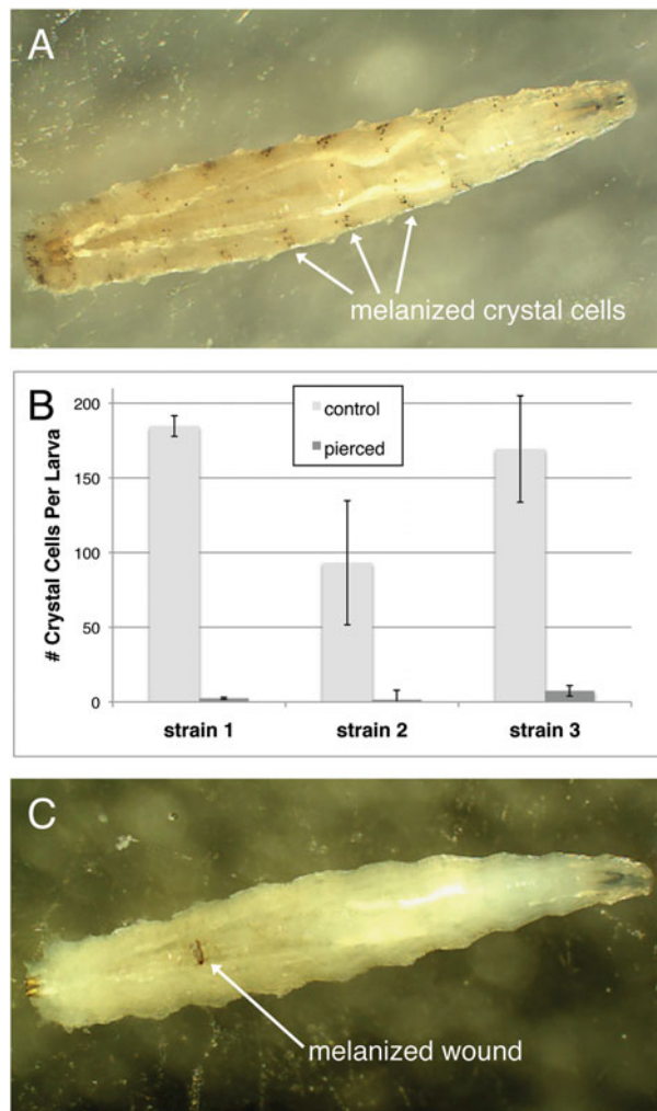
Fig. 13. Zaprionus indianus crystal cells. Fly larvae were incubated to reveal melanized cells, presumably homologous to D. melanogaster crystal cells (A). The mean ( \pm ) standard error numbers of crystal cells were counted in control and pierced larvae from the three Z. indianus strains in three replicates each (B). Pierced, incubated fly larvae show melanized wounds and few melanized crystal cells (C).
