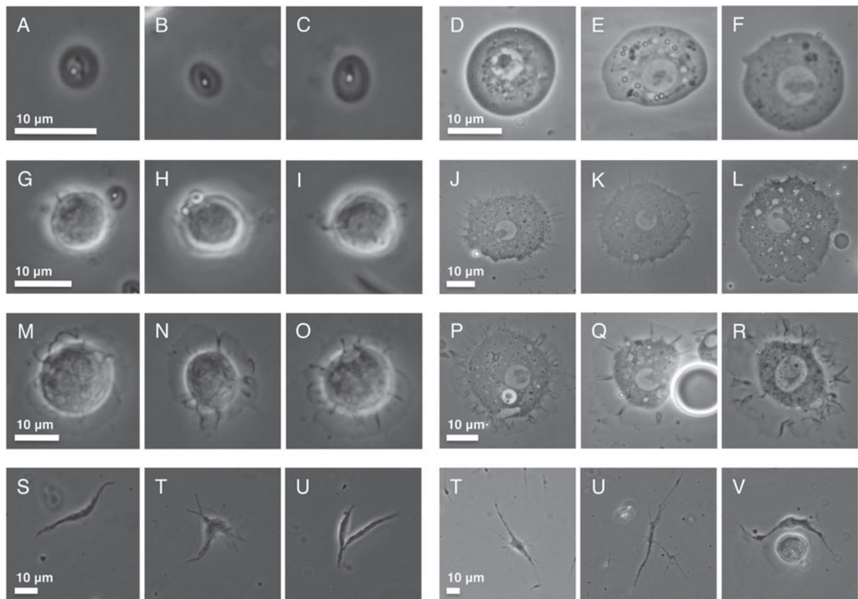
Fig. 9. Zapriomus indianus haemocytes. Cells were dissected onto slides in 1 \times PBS buffer (A–C, G–I, M–O, S–U) or high density immersion oil (D–F, J–L, P–R, T–V). Six representative images are shown for plasmatocytes (A–F), podocytes (G–L), lamellocytes (M–R) and nematocytes (S–V). Size bars are consistent within treatments but note size bar variation across cell types and treatments.
