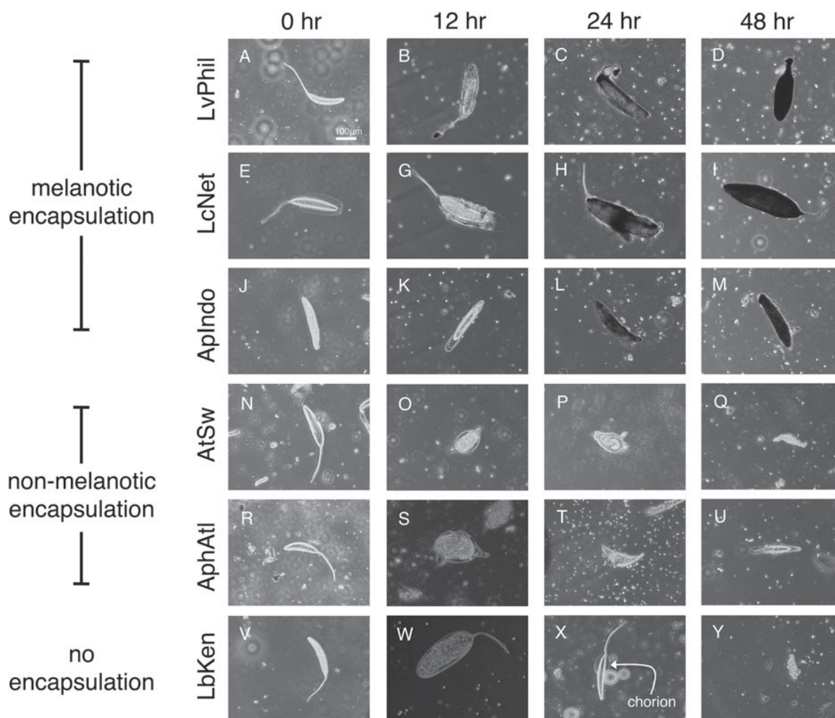
Fig. 8. Three wasp egg-killing strategies used by Z. indianus . Time course images were taken of wasp eggs dissected from infected fly larvae. Zaprionus indianus killed eggs of some wasp species using melanotic encapsulation (A–M), eggs of other wasp species using non-melanotic encapsulation (N–U), and appear to kill L. bouleardi eggs using a non-cellular mechanism of dissolving away the egg chorions (V–Y).
