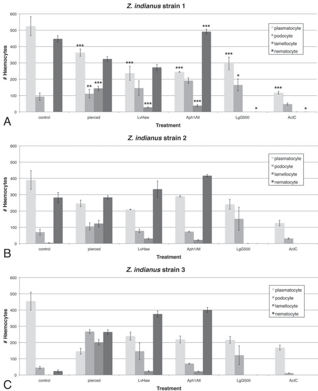
Fig. 11. Constitutive and induced haemocyte numbers in Z. indianus . Control flies were treated like pierced flies but were not pierced; flies were also infected by four wasp strains that showed varying infection success in eclosion trials. The mean ( \pm ) standard error are shown for Z. indianus strains 1 (A), 2 (B), and 3 (C) based on five control and pierced replicates and three wasp-attack replicates. Significant differences between the control and each immune treatment for each cell type, using combined fly strain data, are shown in (A) with * <0.05 , ** <0.01 and *** <0.001 .
