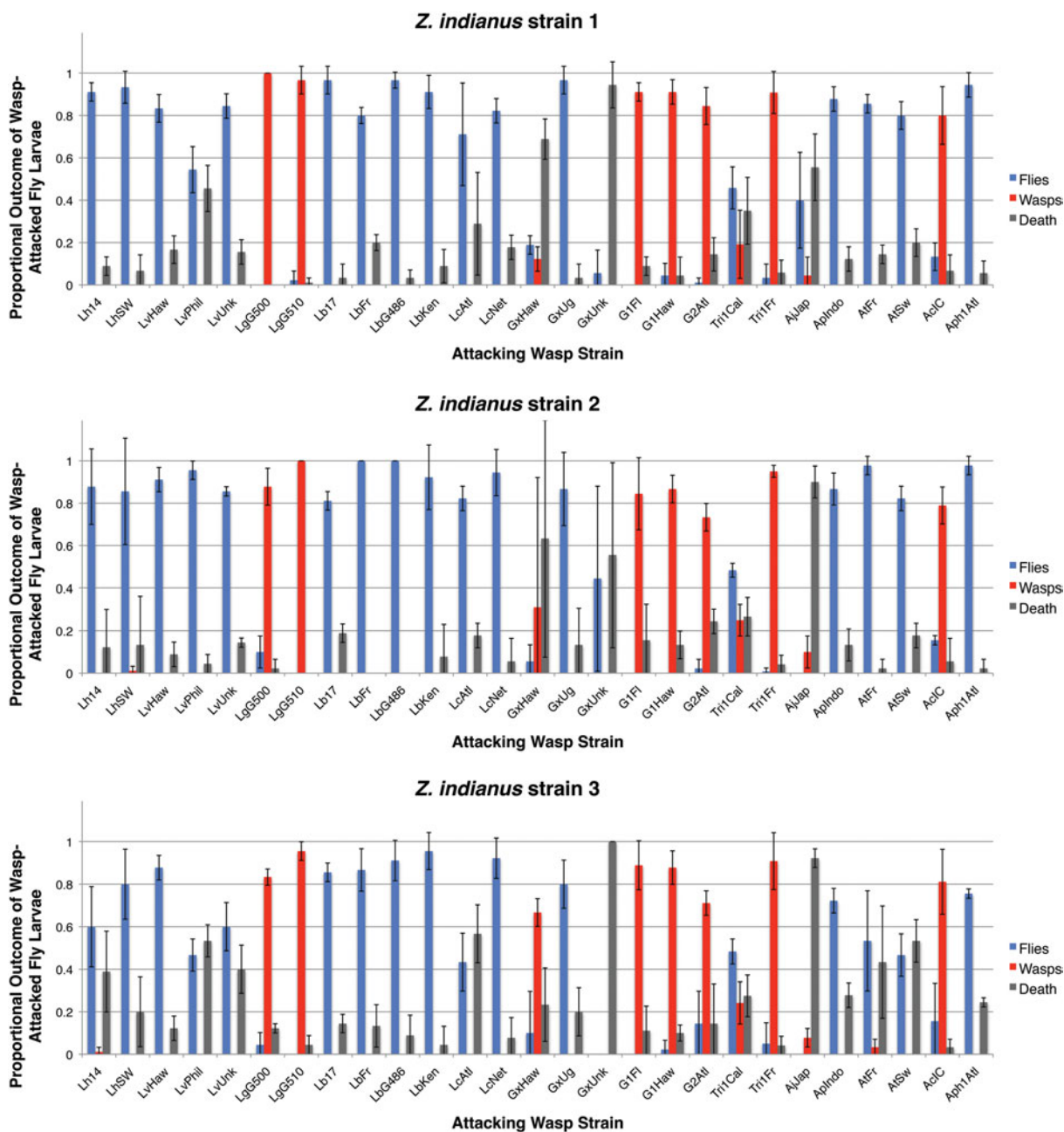
Fig. 4. Outcomes for wasp-infected Z. indianus . The proportion of flies and wasps that eclosed from each fly–wasp interaction, as well as the proportion of wasp-infected flies that died, is shown for Z. indianus strains 1 (A), 2 (B), and 3 (C). The mean ( \pm ) 95% confidence intervals are shown for three replicates of each fly–wasp pair.
