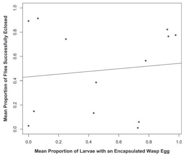
Fig. 7. Lack of correlation between fly encapsulation success and eclosion success. The mean proportion of infected Z. indianus larvae that encapsulated at least one wasp egg was compared to the mean eclosion success of Z. indianus against each wasp, using combined data from the three Z. indianus strains. Data from wasp species strains were averaged into single species values, and pupal endoparasitoids were not considered.
