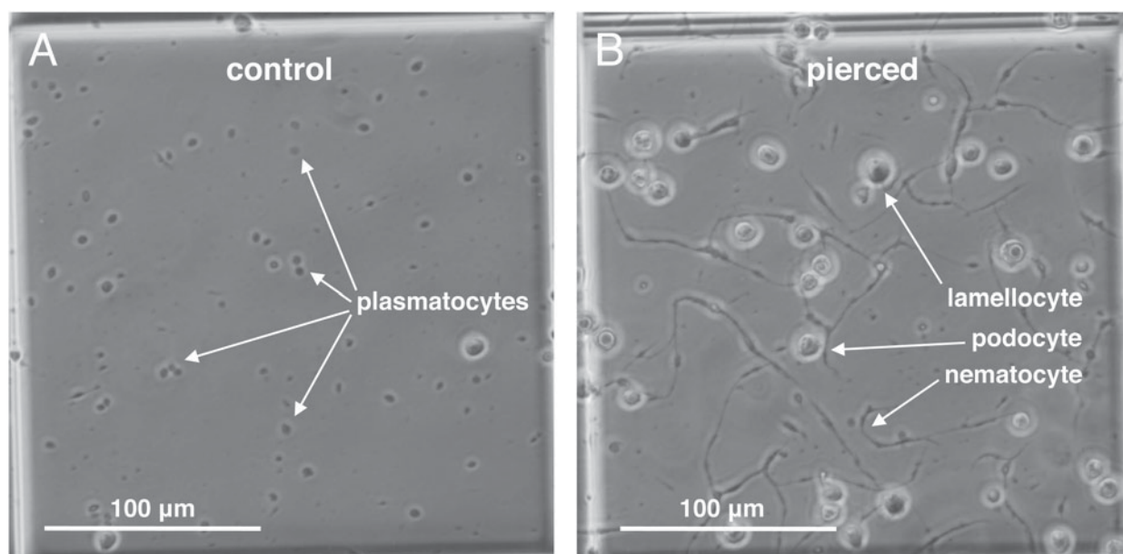
Fig. 12. Induced production of nematocytes and other haemocyte types in Z. indianus strain 3. Haemocytes are visualized in a 0.25 \times 0.25 \times 0.1 mm haemocytometer field. In control flies (A) plasmatocytes are most numerous but 24 h after piercing (B) the numbers of podocytes, lamellocytes and nematocytes increase.
