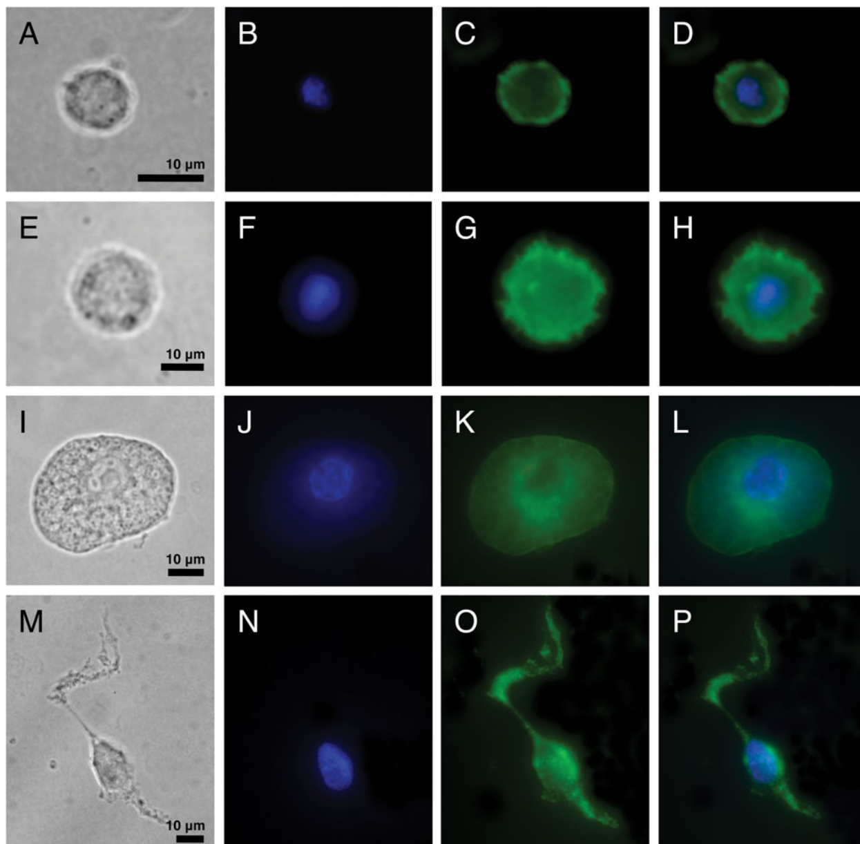
Fig. 10. Zaprionus indianus haemocyte cytoskeletal and nuclear staining. A plasmatocyte (A–D), podocyte (E–H), lamellocyte (I–L), and nematocyte (M–P) are shown, in bright light (A, E, I, M), with DAPI nuclear staining (B, F, J, N), with TRITC-phalloidin actin staining (C, G, K, O), and with merged DAPI and TRITC-phalloidin stains (D, H, L, P). Note that haemocyte morphology differs somewhat from that shown in Fig. 9 due to the cell fixation process.
