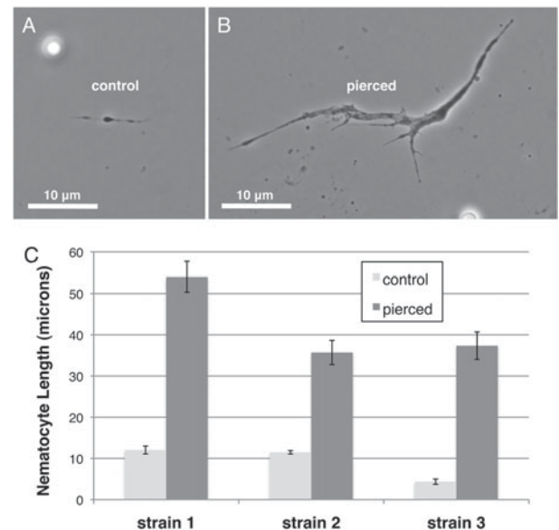
Fig. 14. Constitutive and induced nematocyte length in Z. indianus . Nematocytes in un-induced flies (A) are much shorter and often show less branching than in wasp-attacked flies (B). The mean ( \pm ) standard error of nematocyte lengths from control and pierced flies (C) are based on three control and pierce replicates.
