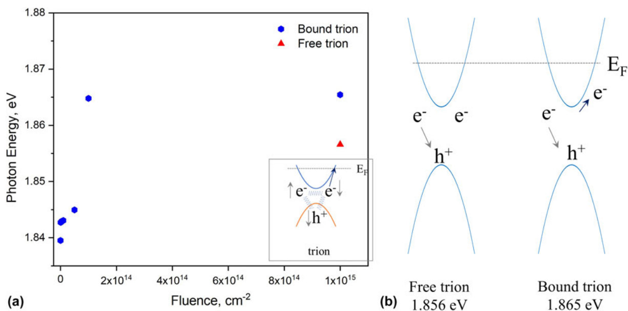
Figure 5: (a) Dependence on ion fluence of the trion peaks and (b) corresponding schematic illustration of the bound and free trions in MoS 2 . The inset in (a) is a schematic representation of the location of electrons and a hole in respect to Fermi energy level in trion.
