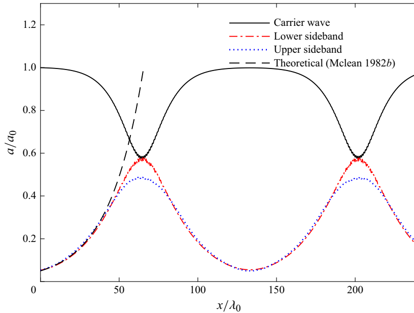
Figure 1. Computed spatial evolution of the carrier wave and sideband amplitudes from the simulated Benjamin–Feir instability for k_0 h = 2\pi with low initial steepness k_0 a_0 = 0.1 . The theoretical sideband growth rate corresponds to the evolution predicted by McLean (1982b).
