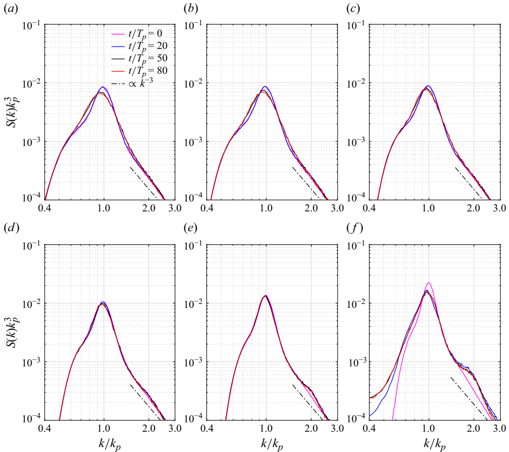
Figure 7. Evolution of the computed spectra for the cases involving six dimensionless water depths.
