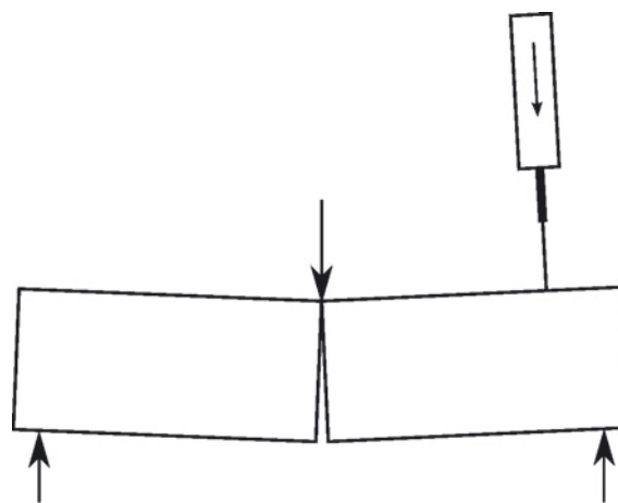
Fig. 7. Schematic of paired tests of tensile strength and blade hardness. The snow sample was first broken in three- or four-point bending (three-point bending shown). Next, a blade hardness measurement was taken (upper right) using a part of the sample that experienced low stress during the strength test.
