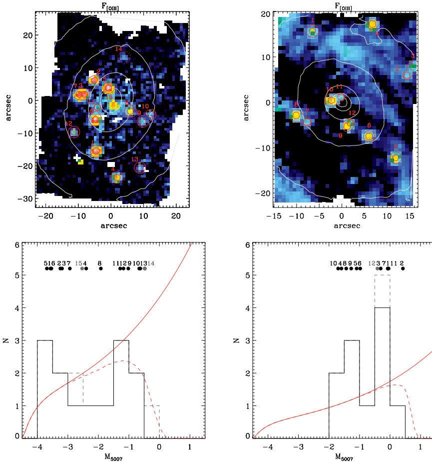
Figure 1. SAURON maps for the flux of the [O III]λ5007 emission (upper panels) from the central regions of M32 (left) and the nuclear regions of M31 (right) together with the luminosity function of the PNe found in them (lower panels). In the [O III] maps the white contours outline the galaxy stellar isophotes whereas the position of the detected PNe is shown by the red contours. The absolute magnitude of these PNe can be read in the lower panels, where the red solid and dashed lines also show the theoretical form of the PNLF (from Ciardullo et al. 1989) as it is and after accounting for the incompleteness of our observations, respectively. Grey points and dashed histograms correspond to marginal PNe detections. In the case of M32, the models have been normalised to match the observed number of PNe to the number of objects that we would expect to detect according to the incompleteness-corrected PNLF model. For M31 the nuclear PNe population is unlikely to have been drawn from such a PNLF model, and the lines are shown mostly for an illustrative purpose and are normalised by simply assuming the same specific PNe density of M32.
