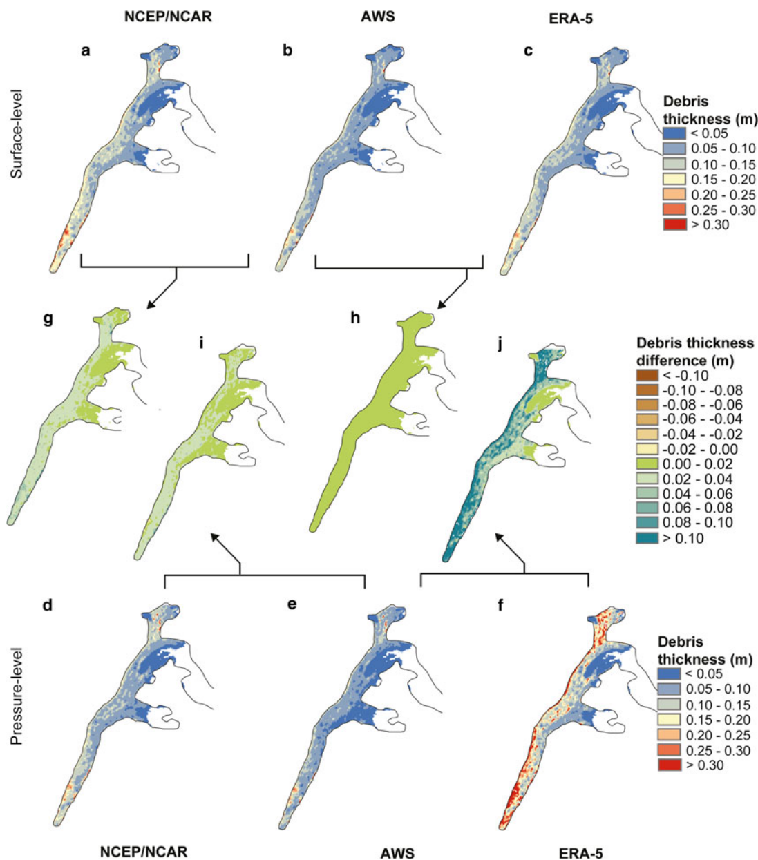
Fig. 6. Distributed debris thickness maps for Khumbu Glacier on 17 June 2009. Figures (a–c) show distributed thickness values derived using surface-level reanalysis data, and (d–f) show distributed thickness values derived using pressure-level data for both ERA and NCEP/NCAR. Figures (g–h) and (i–j) show debris thickness changes relative to the AWS-derived debris thickness control maps.
