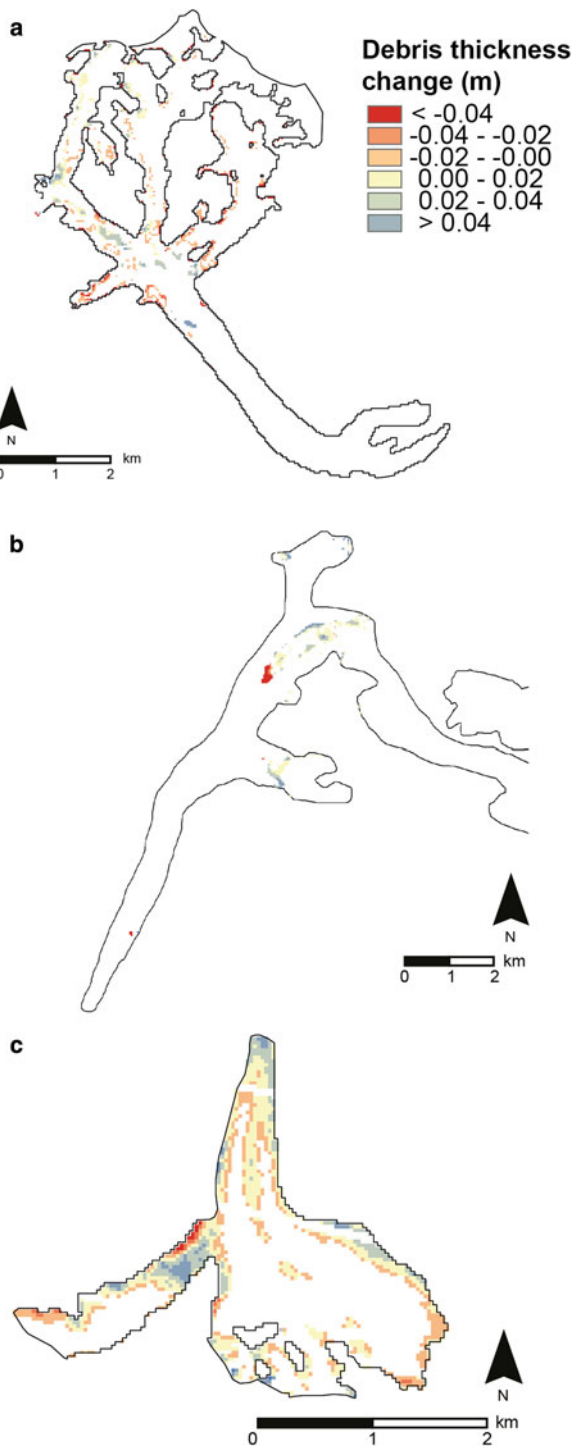
Fig. 11. Significant debris thickness change in meters between (a) 2001–19 (Miage Glacier), (b) 2002–16 (Khumbu Glacier) and (c) 2002–19 (Haut Glacier d'Arolla) derived from ERA surface-level reanalysis data. Distributed maps are derived by differencing the first and last debris thickness estimates at the dates listed above. Where the debris thickness change is below the pixel-specific uncertainty or there is a lack of thermal satellite data, the pixels are coloured white and have been excluded from any further analysis. Glacier outlines are taken from RGIv.6.0 (RGI Consortium, 2017), except for the outline for Haut Glacier d'Arolla which has been updated to reflect the significant retreat of the glacier outline by 2019.
