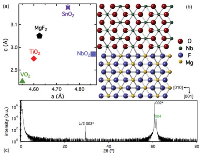
Fig. 2: (a) Plot of the lattice parameters, a and c , of common crystals with the rutile structure including NbO 2 . (b) Schematic cross-section of the epitaxial configuration of a NbO 2 (001) film on a MgF 2 (001) substrate, where niobium atoms are represented by relatively small dark green atoms, oxygen by large dark red atoms, magnesium by small light yellow atoms, and fluoride by larger light purple atoms. (c) \theta -2 \theta x-ray diffraction spectrum of an NbO 2 (001) film on a MgF 2 (001) substrate with “*” denoting peaks arising from the substrate.
