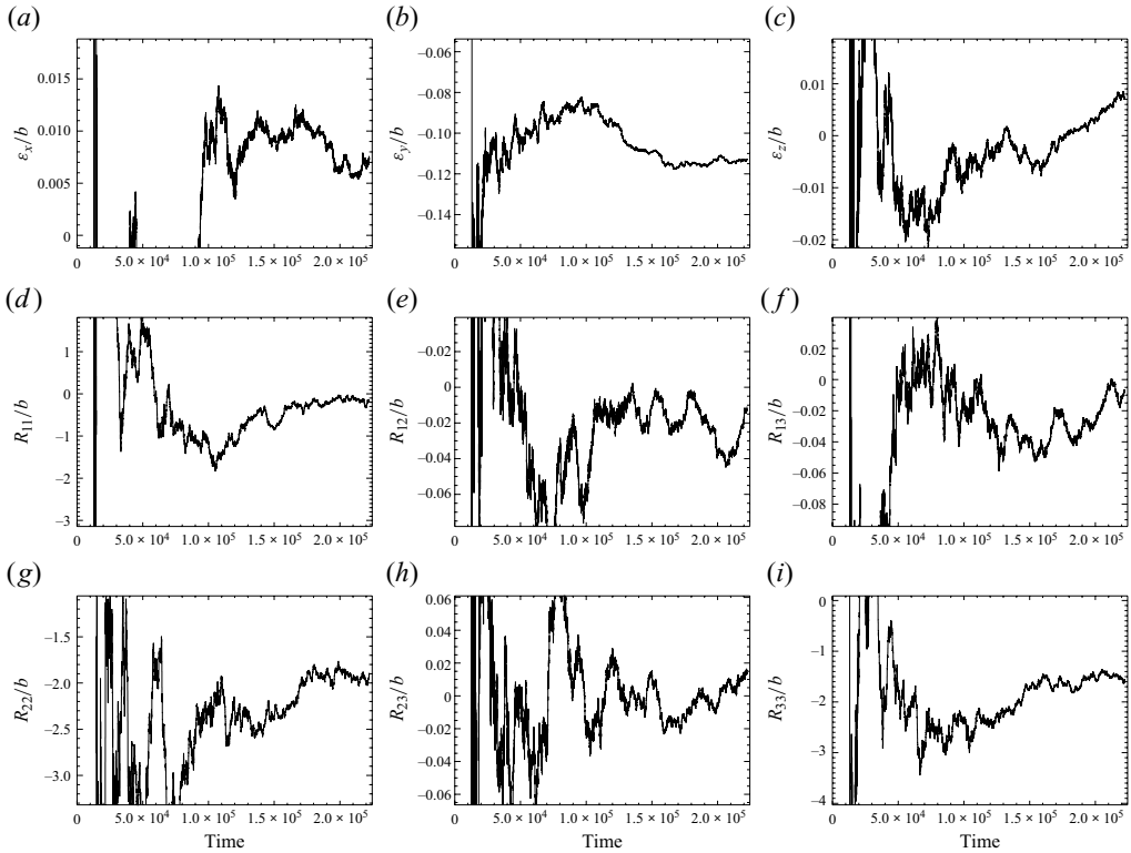
Figure 10. Cumulative averages of the components of the mean e.m.f. ( a–c ) and mean total stress ( d–i ), normalised by the mean field strength b = |\bar{\mathbf{b}}| , calculated from the nonlinear MHD equations, with forcing F_1 and Re = Rm = 100 , after the imposition of a mean magnetic field \bar{\mathbf{b}} = 10^{-3}\hat{\mathbf{y}} .
