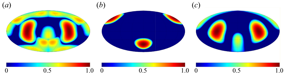
Figure 4. Mollweide (\theta, \phi) projections of the scaled growth rate (the largest value of |\text{Im}(\omega)|/|\mathbf{K}| ), for the system described by (3.14), (3.15); longitude is in the range -\pi < \phi < \pi , latitude in the range 0 < \theta < \pi (the equator is \theta = \pi/2 ): (a) growth rate for the full system, governed by the matrix (3.16); (b) growth rate for the system in which only the \alpha^{(1)} effect operates ( \mathbf{Q}^{(1)}, \mathbf{Q}^{(2)}, \mathbf{R}^{(2)} all zero); (c) growth rate for the system in which only the \Gamma^{(1)} effect operates ( \mathbf{Q}^{(2)}, \mathbf{R}^{(1)}, \mathbf{R}^{(2)} all zero). In each plot, the maximum of the scaled growth rate is normalised to unity; the numerical values of the maximum scaled growth rate are (a) 0.338, (b) 0.267 and (c) 0.338.
