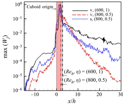
Figure 14. Streamwise variation of the maximum of the wavemaker for the leading varicose mode in case (Re_h, \eta) = (600, 1) , and the leading varicose and sinuous modes in case (Re_h, \eta) = (800, 0.5) . The vertical dashed lines denote the locations of cuboid origin and edges of the reversed flow regions.
