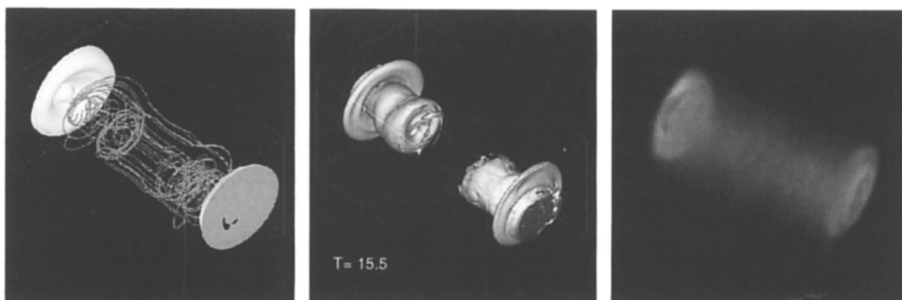
Figure 1. Numerical results for a typical model with \beta = 100 at t = 15.5r_0/V_{K0} . The left panel shows the density isosurface and magnetic field lines. The middle panel shows the isosurface of magnetic field strength B/B_0 = 10 . The right panel is the pseudo X-ray image rendered by using \rho^2 T^{1/2} .
