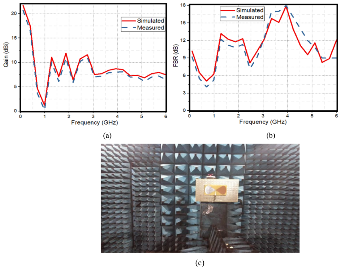
Figure 12. Simulated and measured (a) gain and (b) FBR; (c) anechoic chamber photograph.
