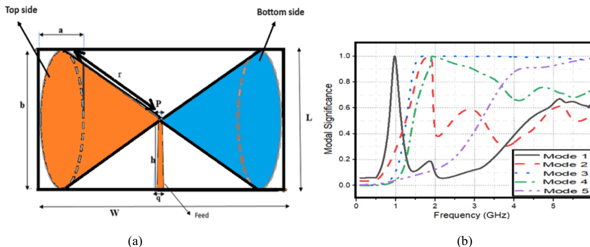
Figure 1. Proposed bowtie antenna. (a) Schematic and (b) MS values.
