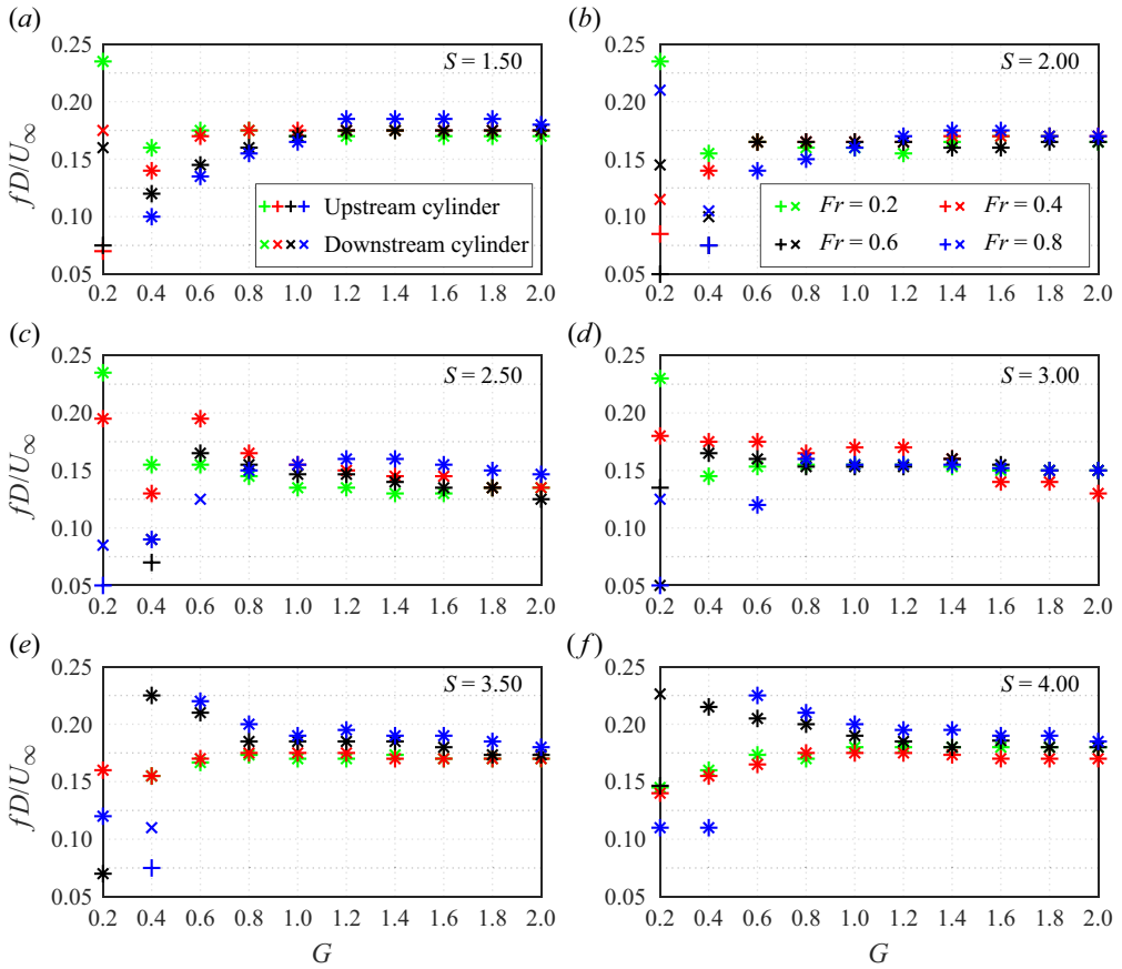
Figure 20. Variations of Strouhal numbers for the two tandem cylinders as a function of gap ratios at (a) S = 1.5 , (b) S = 2.0 , (c) S = 2.5 , (d) S = 3.0 , (e) S = 3.5 and (f) S = 4.0 .
