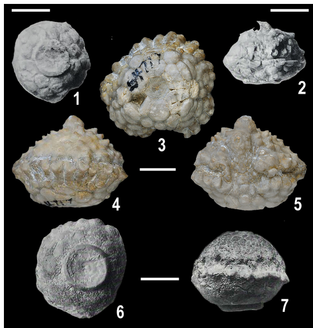
Figure 10. Paragaricocrinids. (1, 2) Nipponicrinus akiyoshiensis n. gen. n. sp. (ASM 50058), holotype, scale bar represents 10.0 mm; images from Hashimoto (2001), used with permission; (1) basal view of calyx, (2) lateral view of calyx. (3–5) Pulcheracrinus exotericus (Strimple, 1951) n. gen. n. comb. (USNM PAL 4717), scale bar represents 5.0 mm; images courtesy of the Smithsonian Institution, GUID: http://n2t.net/ark:/65665/39b179562-3e0a-4c14-b245-c827fdb712d1 ; (3) basal view of calyx, (4) A-ray lateral view of theca, (5) CD-interray lateral view of theca. (6, 7) Nipponicrinus hashimotoi n. gen. n. sp. (ASM 50053), holotype, scale bar represents 10.0 mm; images from Hashimoto (2001), used with permission; (6) basal view of calyx, (7) lateral view of calyx.
