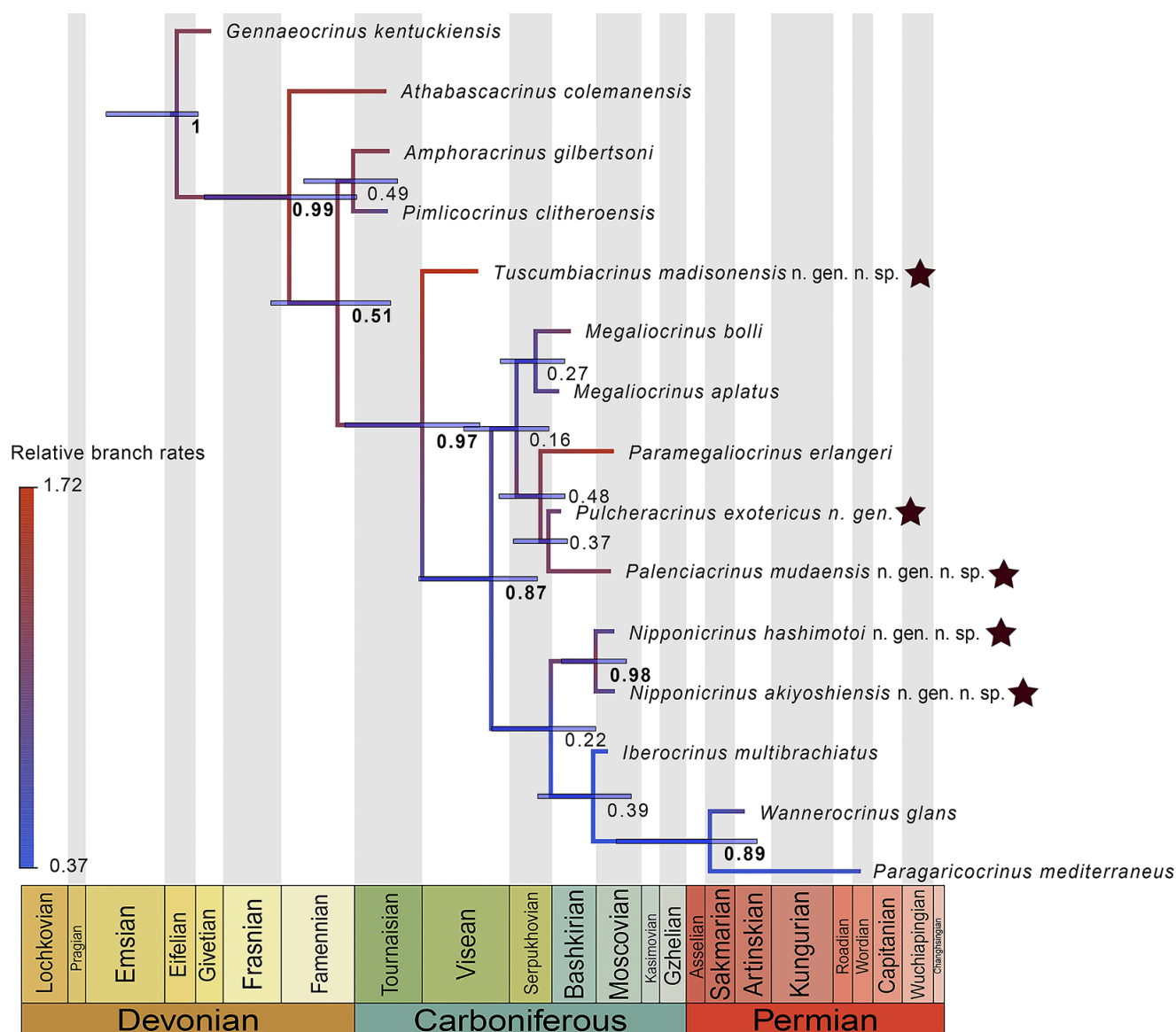
Figure 6. Paragarcicrinidae phylogeny from Bayesian tip-dating analysis. Stars indicate new and/or revised taxa; numbers correspond to the posterior probabilities of clades; branches are colored to show relative rates of morphological evolution. Taxonomic names are those from results of this study.
