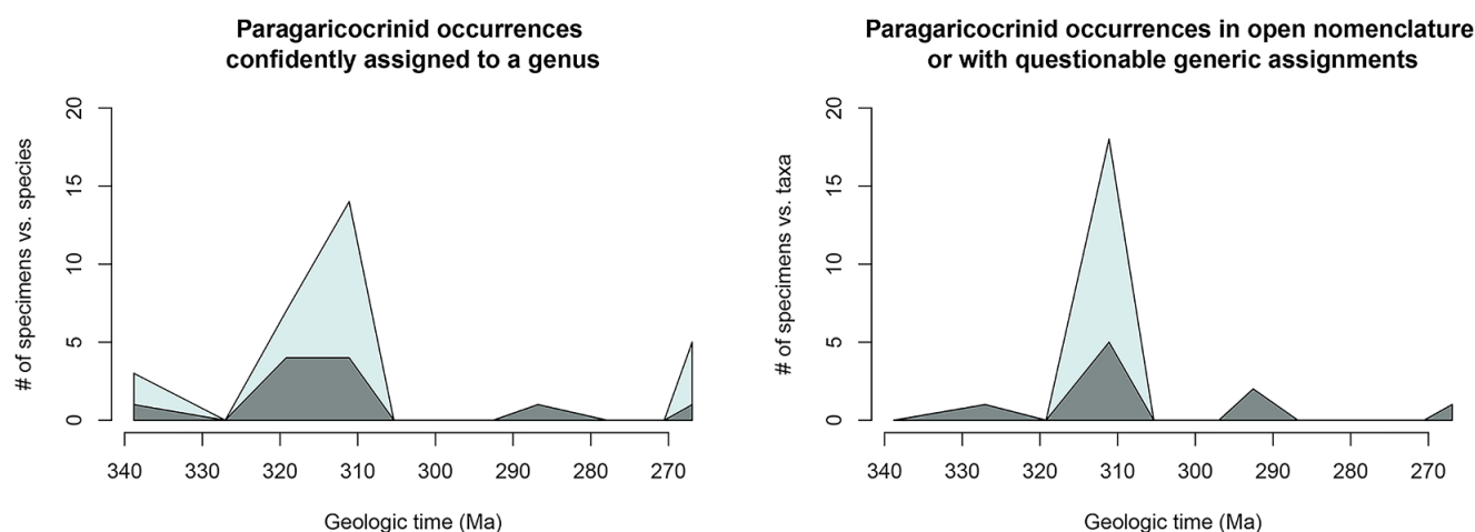
Figure 8. Comparison of the number of species (dark blue) to number of specimens (light blue) for species of paragarcocrinids (left) that are confidently assigned to a genus and (right) for species questionably assigned to a genus and those left in open nomenclature.
