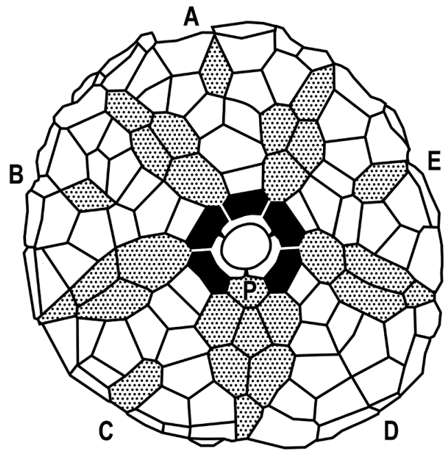
Figure 9. Plate diagram of Tuscumbiacrinus madisonensis n. gen. n. sp. Radial plates black, interradial and intraradial plates stippled, and P designates the primanal.
