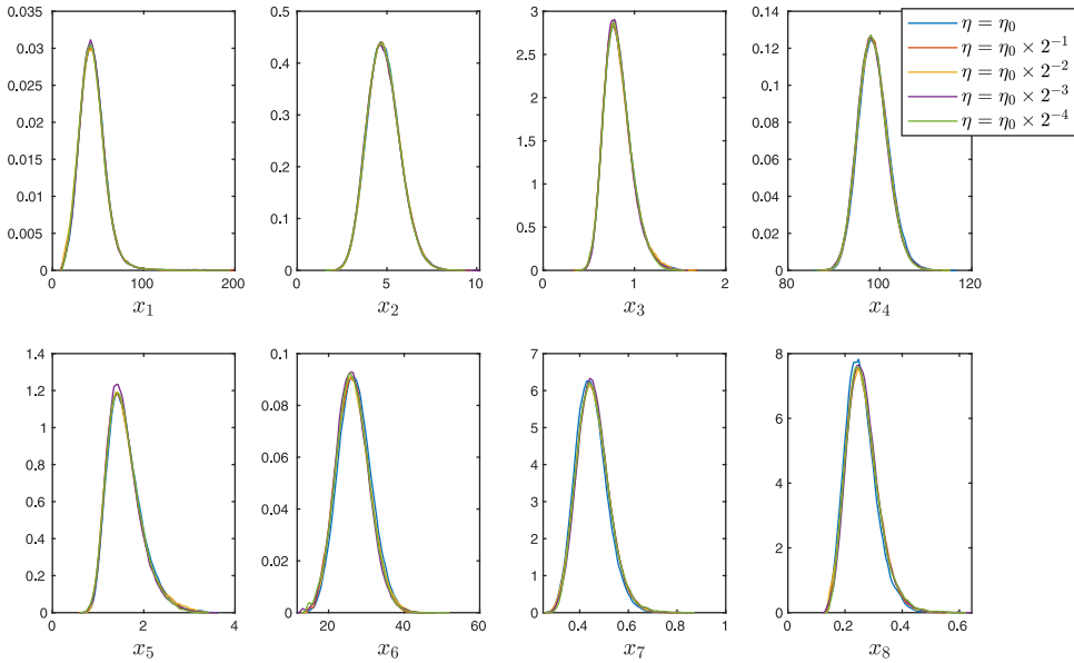
FIGURE 2. Marginal distributions of perturbed posteriors defined by various time step sizes.
