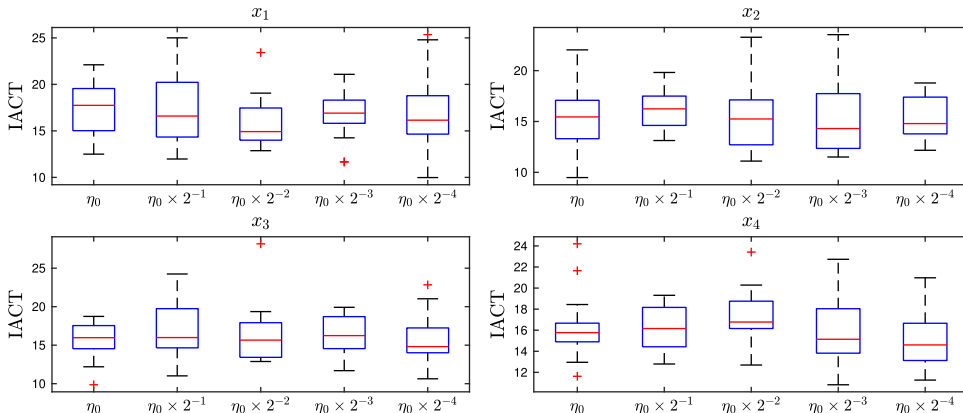
FIGURE 5. Box plots of integrated autocorrelation times (IACTs) of the first four parameters of Markov chains simulated by Algorithm 1. Here, 20 realizations of Markov chains are used to estimate the IACT.
