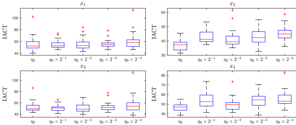
FIGURE 4. Box plots of integrated autocorrelation times (IACTs) of the first four parameter Markov chains simulated by the MALA algorithm. Here, 20 realizations of Markov chains are used to estimate the IACT.
