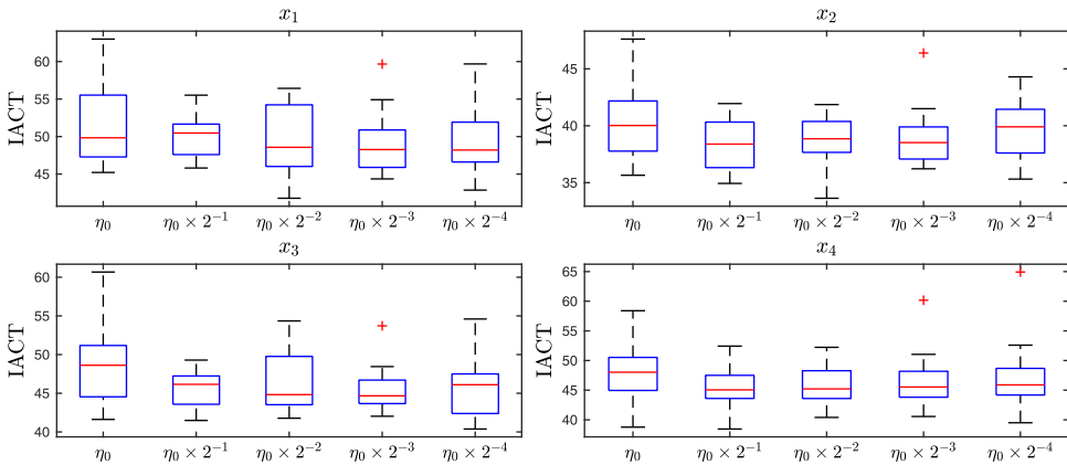
FIGURE 3. Box plots of integrated autocorrelation times (IACTs) of the first four parameter Markov chains simulated by the RWM algorithm. Here, 20 realizations of Markov chains are used to estimate the IACT.
