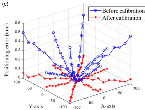
Figure 9. Positioning error distribution of the moving platform.
