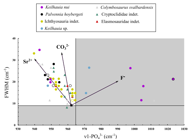
Figure 7. The \nu_1(PO_4^{3-}) stretching band position and full width at half maximum (FWHM) measured for Ichthyosauria and Plesiosaurs bones and teeth (Supplementary Table 3). Empty symbols represent enamel samples, while solid symbols represent bone samples. The gray zone corresponds to the combination of parameters that would indicate a mineralogical alteration of the bioapatite of teeth and bones. The black arrows indicate the evolution of the position of the \nu_1(PO_4^{3-}) stretching band position and the FWHM depending on the type of ionic substitution within the bioapatite (Thomas et al. 2011).
