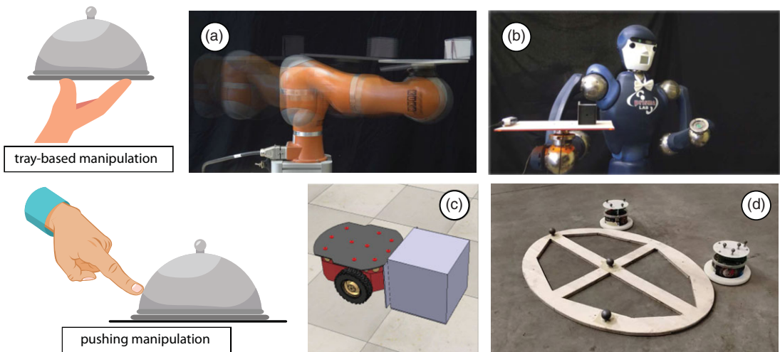
Figure 2. Tray-based and pushing non-prehensile object manipulation scenarios. Upper row: a robot is tasked with transporting an object placed on a tray-like end-effector along a predefined, fast trajectory while avoiding the relative sliding (a) [20]. The robot performs a linear transporting trajectory while opportunely inclining the tray to improve the robustness of the task performance (b) [19]. Bottom row: an object is pushed by a mobile robot along a trajectory (c) [16]. Multiple robots can push an object with minimal effort by optimally placing themselves around it (d) [17].
