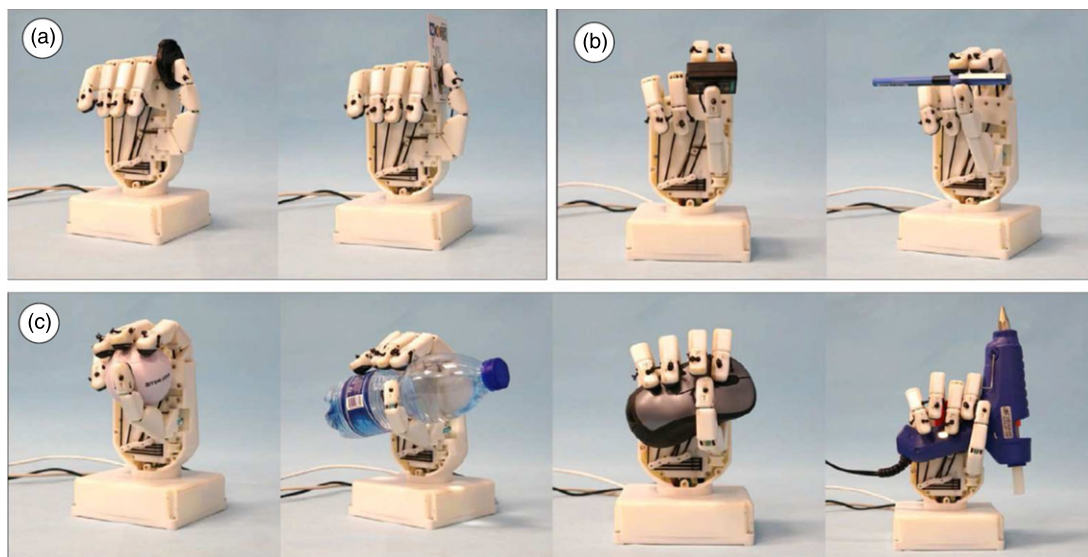
Figure 9. The PRISMA Hand II and its capabilities. The grasping options are categorized into three sets: (a) lateral grasps, (b) pinches, and (c) power grasps [154, 155].
