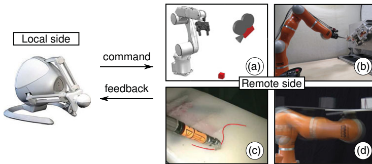
Figure 6. A shared control telerobotic system consists of a local device used to jointly send partial commands and receive computed haptic information as feedback from the remote side. The user usually observes the remote environment by means of a camera that provides a limited awareness of the scene. In (a), the robot must execute a remote object grasping task [91]. In this case, provided haptic information aims to increase the situational awareness of the operator informing about the proximity to the robot's joint limits and singularities. In (b) and (c), vision-based or programmed virtual fixtures aid the execution of the task in industrial and surgical robotic settings, respectively [92, 93]. In (d), a non-prehensile object transportation scenario is considered and haptic feedback is provided about the proximity to the sliding conditions of the object placed on the tray [19].
