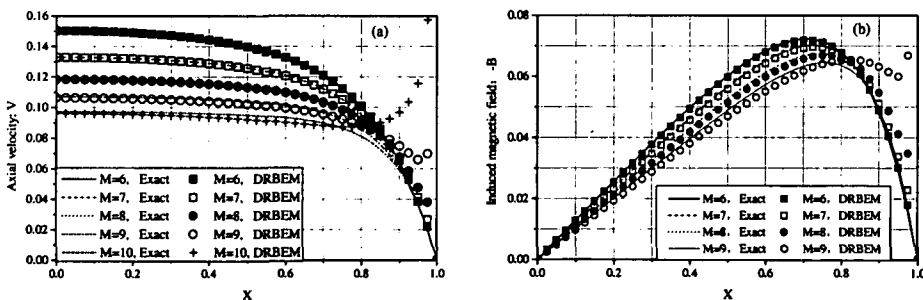
FIGURE 7. (a) Profiles of V along the x -axis of the rectangular channel with \phi = \pi/2 and \lambda = \infty for M = 6, 7, 8, 9, 10 ; (b) profiles of -B along the x -axis of the rectangular channel with \phi = \pi/2 and \lambda = \infty for M = 6, 7, 8, 9 .
