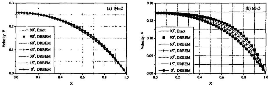
FIGURE 1. Profiles of the axial velocity along the x -axis of a rectangular channel in the presence of the magnetic field applied to the channel with various angles \phi for a non-conducting wall; (a) M = 2 , (b) M = 5 .
