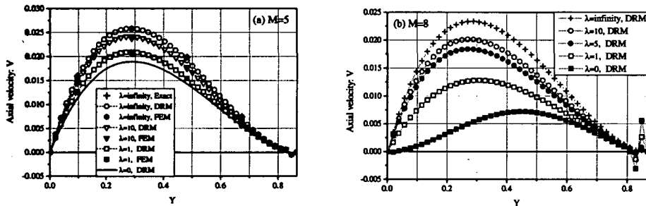
FIGURE 13. Profiles of the axial velocity V along the y -axis of a triangular channel for arbitrary wall conductivity and \phi = \pi/2 ; (a) M = 5 , (b) M = 8 .
