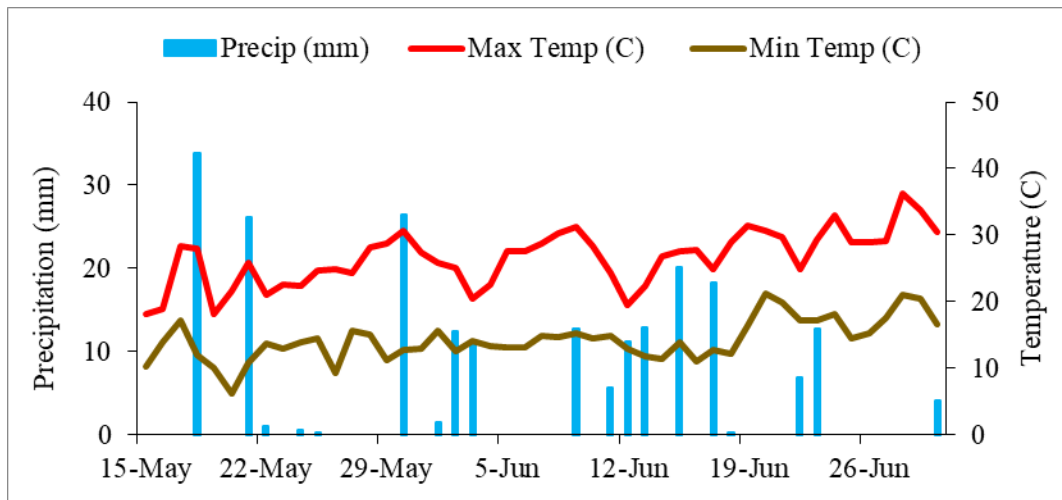
Figure 2. Daily minimum and maximum air temperature (C) and precipitation (mm) during the growing season at Kansas State University Southwest Research and Extension Center (KSU-SWREC) near Garden City, KS.
