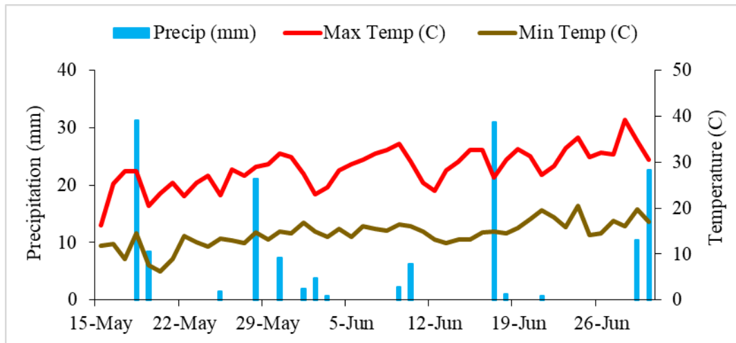
Figure 1. Daily minimum and maximum air temperature (C) and precipitation (mm) during the growing season at Kansas State University Agricultural Research Center (KSU-ARC) near Hays, KS.
