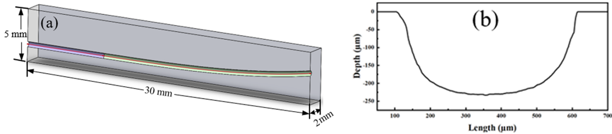
Figure 1. Design of the curved capillary: (a) schematic view of the curved plasma channel on a sapphire substrate; (b) typical cross-section of the laser etched channel on the substrate.
