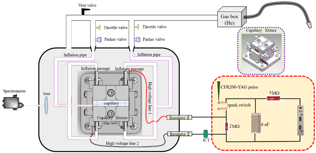
Figure 2. Schematic diagram of a plasma channel generated by high-voltage discharging of a gas-filled capillary.
