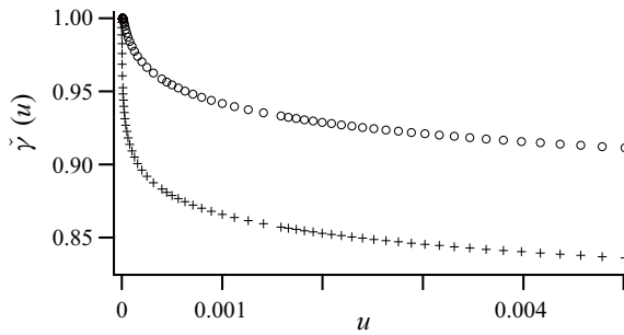
FIGURE 2. We plot \check{\gamma}(u) for \tau = 1.008 \times 10^{-3} (o) and 1.26 \times 10^{-4} (+). As mentioned in the text, \check{\gamma} represents the drag coefficient non-dimensionalized by (2.9), while u represents the particle speed non-dimensionalized by U^* \equiv s^*r_0 .
