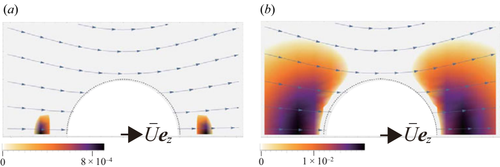
FIGURE 5. Colour gradation represents the largest of zero and 1 - \frac{\tau}{\tau_{s(0)}} v^{(d-z)} for c = 1 and U = \bar{U} at each of \tau = 1.26 \times 10^{-2} (a) and 8.064 \times 10^{-3} (b). The particle is assumed to move translationally with the velocity \bar{U}e_z . The region shown in each figure is the same as in figure 1; the dotted curve represents the half of the cross-section of the particle surface. The curves outside the particle are the stream lines of v^{(0)} , which are represented by arrows in figure 1.
