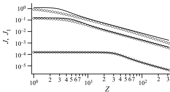
FIGURE 8. From the top, three solid curves, respectively, represent J_1(1.0, Z) , J_1(0.5, Z) and J_1(0.05, Z) , while three series of circles, respectively, represent J(1.0, Z) , J(0.5, Z) and J(0.05, Z) . We calculate J(q, Z) by means of numerical integration in Mathematica (Wolfram Research) with Method \rightarrow {'GlobalAdaptive', 'MaxErrorIncreases' \rightarrow 10 000, Method \rightarrow 'GaussKronrodRule'}, MaxRecursion \rightarrow 20.
