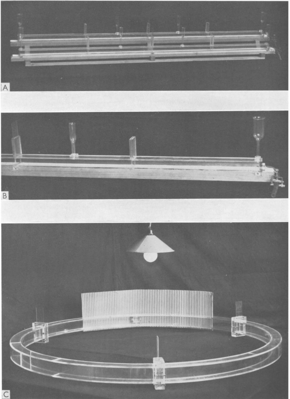
A. General view of second Perspex horizontal apparatus. B. Detail of right-hand half of one tube of above. C. Perspex horizontal circular apparatus, showing the three sliding doors, one section of a surrounding cardboard shield and the electric light.
