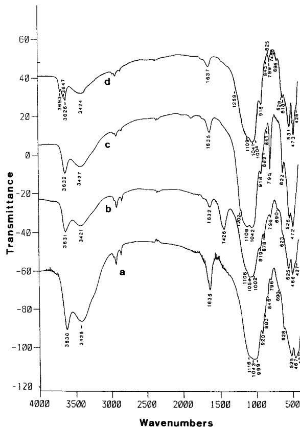
Figure 9. Representative IR spectra of smectites (less than 2 \mu\text{m} fraction) present in the Milos bentonites. a = Ankeria deposit, b = Aspro Horio deposit. c = Ano Komia deposit, d = Agrilies deposit.
