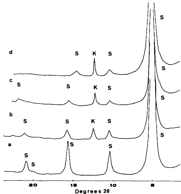
Figure 4. Representative XRD patterns of the less than 2 μm clay fractions. a = Ankeria deposit, b = Tsantili deposit, c = Garyfalakena deposit, d = Agrilies deposit. Key to the letters: S = smectite, K = kaolinite.
