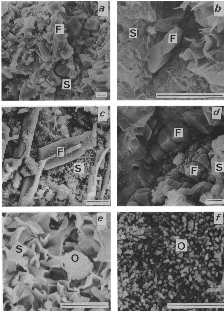
Figure 8. Authigenic K-feldspar (a–d) and opal-CT (e–f) textures observed in the Miloan bentonites: In photos a, b and d K-feldspar crystals (F) fill dissolution cavities being associated with smectite (S). In photo c euhedral K-feldspar crystals (F) are draped over smectite (S) groundmass. a = Koufi deposit, b = Ankeria deposit, c = Tsantili deposit, c = Ano Komia deposit. Photo e: spherulitic opal-CT crystal (O) on smectite flakes (S). Ankeria deposit. Photo f: opal-CT crystals (O) with axiolitic texture. According to Moncure et al (1981) this texture might be the product of direct devitrification of volcanic glass. Garyfalakena deposit. Scale bars: a, c, d, f: 5 \mu\text{m} , b, e: 2.5 \mu\text{m} .
