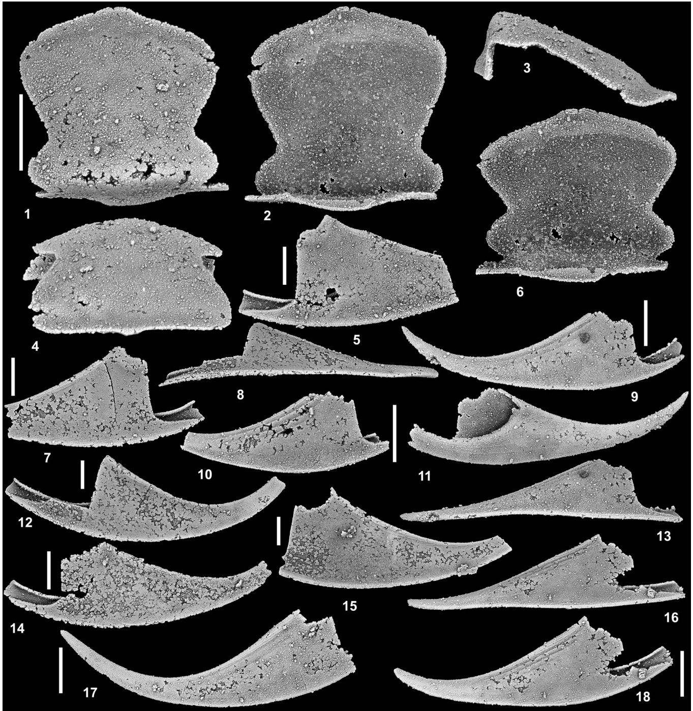
Figure 14. Ibxocephala dekostrae n. gen. n. sp., from Section D 106.4 m, Fillmore Formation (upper Tremadocian, Tulean, high Psalikelopsis cuspidicauda Zone), southern House Range, Ibex area, Millard County, western Utah, USA. (1–4, 6) Cranidium, SUI 148553, dorsal, ventral, right lateral, anterior, and ventral occipital views. (5) Left librigena, SUI 148554, external view. (7) Right librigena, SUI 148555, external view. (8, 12) Left librigena, SUI 148556, ventrolateral and external views. (9, 11, 13) Right librigena, SUI 148557, external, internal, and ventrolateral views. (10) Right librigena, SUI 148558, external view. (14) Left librigena, SUI 148559, external view. (15) Left librigena, SUI 148560, external view. (16, 18) Right librigena, SUI 148561, ventrolateral and external views. (17) Right librigena, SUI 148562, external view. Scale bars = 1 mm.
