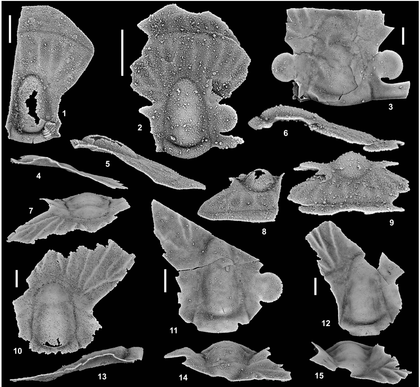
Figure 6. Licnocephala bradleyi n. sp., from Section HC5 225.6 m, east side of Hillyard Canyon, and Section HC6 205.5–224.5 m, west crest of Hillyard Canyon, Garden City Formation (upper Tremadocian, Tulean, Psalikilus hestoni Zone to Protopliomerella contracta Zone), Bear River Range, Franklin County, southeastern Idaho, USA. (1, 5, 8) Cranidium, SUI 148509, dorsal, right lateral, and anterior views (HC6 218.0 m). (2, 6, 9) Cranidium, SUI 148510, dorsal, right lateral, and anterior views (HC6 224.5 m). (3) Cranidium, SUI 148511, dorsal view (HC6 221.5 m). (4, 7, 10) Cranidium, SUI 148512, right lateral, anterior, and dorsal views (HC6 205.5 m). (11, 13, 14) Cranidium, SUI 148513, dorsal, left lateral, and anterior views (HC5 225.6 m). (12, 15) cranidium, SUI 148514, dorsal and anterior views (HC6 224.5 m). Scale bars = 1 mm.
