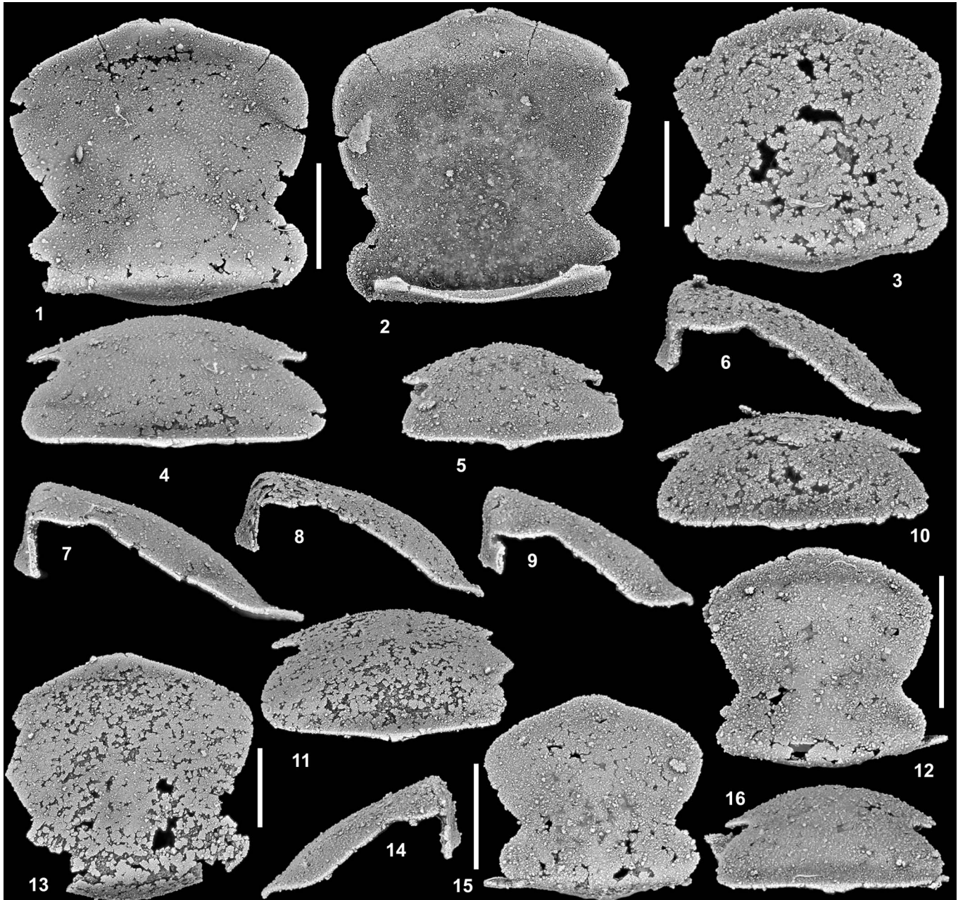
Figure 13. Ibexocephala dekostrae n. gen. n. sp., from Section D 106.4 m, Fillmore Formation (upper Tremadocian, Tulean, high Psalikilopsis cuspidicauda Zone), southern House Range, Ibx area, Millard County, western Utah, USA. (1, 2, 4, 7) Cranidium, holotype, SUI 148548, dorsal, ventral, anterior, and right lateral views. (3, 6, 10) Cranidium, SUI 148549, dorsal, right lateral, and anterior views. (5, 14, 15) Cranidium, SUI 148550, anterior, left lateral, and dorsal views. (8, 11, 13) Cranidium, SUI 148551, right lateral, anterior, and dorsal views. (9, 12, 16) Cranidium, SUI 148552, right lateral, dorsal, and anterior views. Scale bars = 1 mm.
