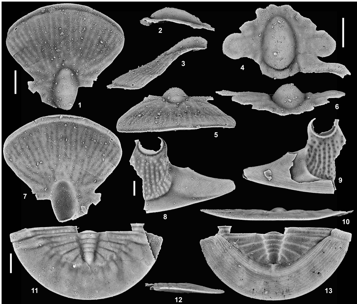
Figure 4. Linocephala ngi n. sp., from Section HC5 195.7 m, east side of Hillyard Canyon, and Section HC6 189.3 m, west crest of Hillyard Canyon, Garden City Formation (upper Tremadocian, Tulean, low Psalikilopsis cuspidicauda Zone), Bear River Range, Franklin County, southeastern Idaho, USA. (1, 3, 5, 7) Cranidium, holotype, SUI 148500, dorsal, left lateral, anterior, and ventral views (HC6 189.3 m). (2, 4, 6) Cranidium, SUI 148501, right lateral, dorsal, and anterior views (HC6 189.3 m). (8, 9) Left librigena, SUI 148502, external and internal views (HC5195.7 m). (10–13) Pygidium, SUI 148503, posterior, dorsal, left lateral, and ventral views (HC6 189.3 m). Scale bars = 1 mm.
