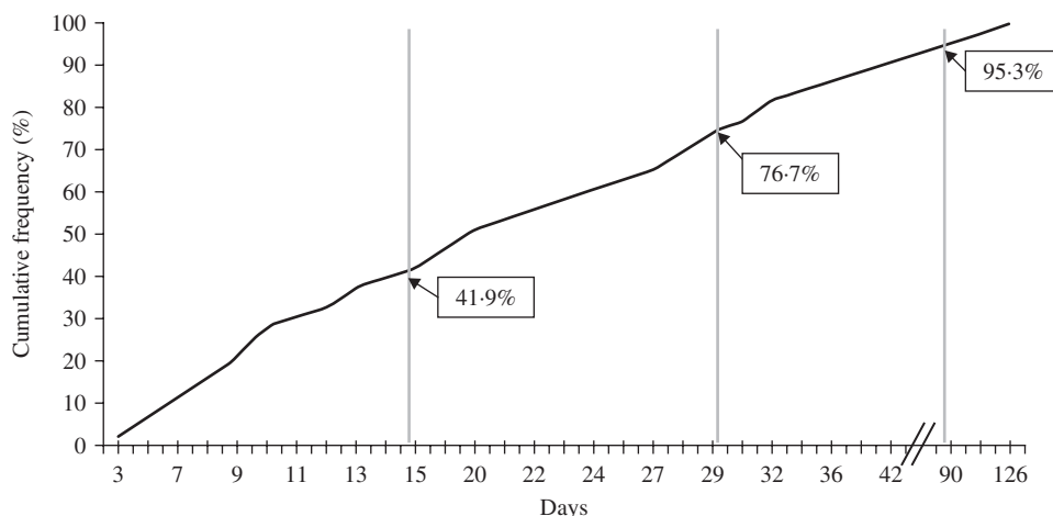
Fig. 1. Cumulative frequency of diagnosed surgical-site infections according to the time interval between the operation and the onset of the infection. Mean length of hospital stay = 15 days (s.d. = 8 days).
