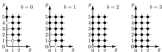
Fig. 1. The behaviour of \Delta_k(\Sigma) when b \leq 3 , g \leq 2 and p \leq 5 . Symbols indicate the behaviour of \Delta_k(\Sigma) as k goes to infinity: solid disks indicate exponential behaviour, striped disks polynomial behaviour, solid circles that \Delta_k(\Sigma) = 1 , and dotted circles represent unsolved cases. Triangles mean that \mathcal{F}(\Sigma) is finite. When b = 0 and there is no symbol, \mathcal{F}(\Sigma) is empty.
