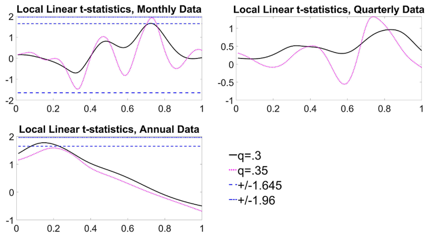
FIGURE 4. Local linear t -statistics for H_0 : \partial \mu(\tau) / \partial \tau = 0 .
