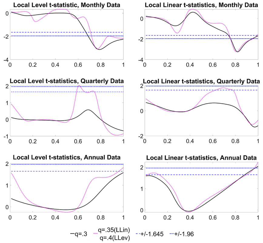
FIGURE 3. Local level/linear t -statistics for H_0 : \beta(\tau) = 0 .
