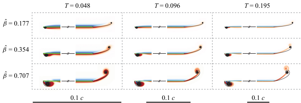
Figure 9. Flat plate. Type-III vortex: m = 0 , p = 0.5 and d = 0 for Re = 32\,000 . Description as for figure 4.
