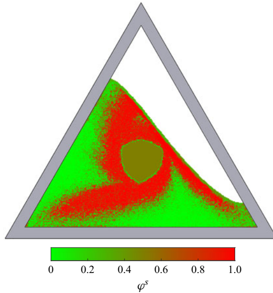
Figure 6. Approximated small-particle concentration field at t = 48 s for the experiment using a triangular drum 70 % filled with an approximately 50:50 mixture of large green and small red glass beads. The small-particle concentration is obtained using the projection method described in § 4.5.
