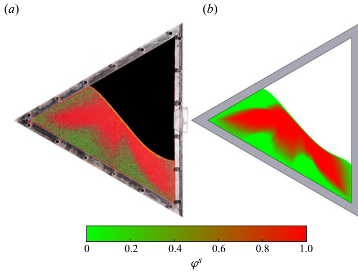
Figure 10. Photo of the experiment (a) and the small-particle concentration in the numerical simulation (b) of a 50% filled drum at t = 42 s containing a 50:50 mix of large green and small red glass beads. Two small-particle arms are distinguishable when the free surface is approximately parallel to the lower drum wall.
