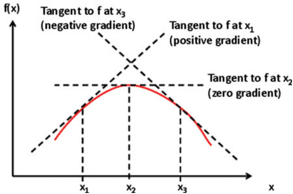
FIGURE 2. (Colour online) The curved red line shows the graph of f as a function of x ; f has a single maximum, at x_2 . We also consider randomly selected points x_1 and x_3 such that x_1 < x_2 < x_3 . The gradient of f at x_1 (respectively, at x_3 ) is positive (respectively, negative); subject to auxiliary structural assumptions, even without e.g. calculating the value of f at x_1, x_3 or anywhere else, or calculating the precise location of the maximum, this information on local gradients would suffice for the correct prediction that x_1 (respectively, x_3 ) is below (respectively, above) the point at which f takes its maximum value.
