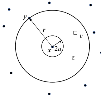
FIGURE 1. Calculation of \bar{h}_2(x, y) . Black dots are particle centres.
