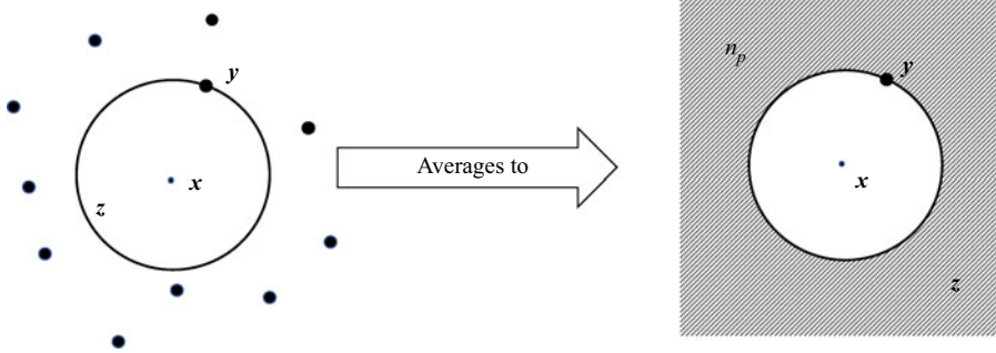
FIGURE 2. Effective medium formed by particles outside the particle-free region.
