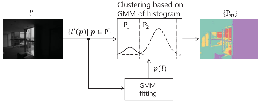
Fig. 2. Proposed image segmentation. Each separated area P_m is color-coded in the right image. Separated areas \{P_m\} are given by the GMM-based clustering method, where GMM is fit by using luminance distribution of input image l .
