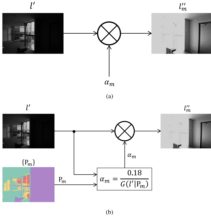
Fig. 3. Proposed segmentation-based exposure compensation, which can automatically calculate M parameters \{\alpha_m\} , although conventional methods cannot. (a) Conventional [19], (b) Proposed.
