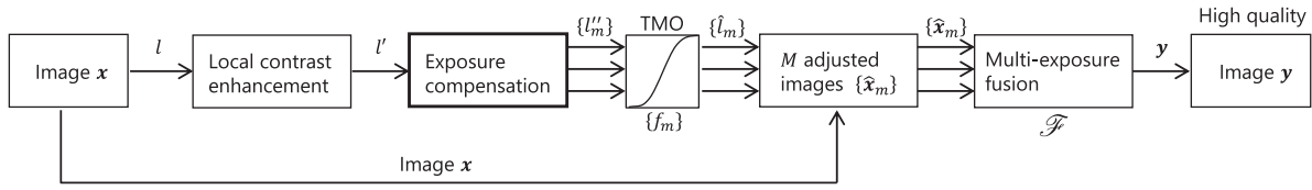
Fig. 1. Pseudo multi-exposure image fusion (MEF). Our main contributions are to propose an image segmentation method to calculate suitable parameters and to propose a novel exposure compensation method based on the segmentation method.
