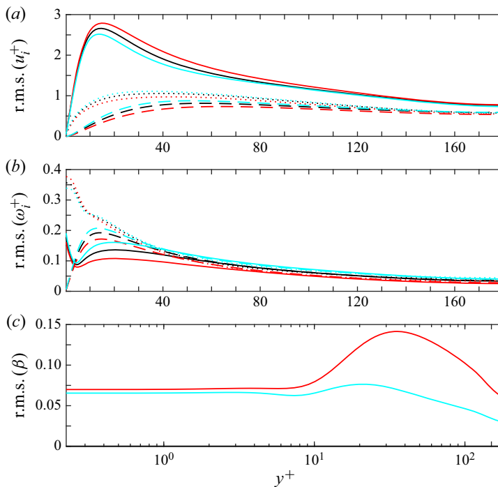
FIGURE 8. Second-order statistics: (a) turbulence intensities \text{r.m.s.}(u_i^+) , (b) r.m.s. values of vorticity fluctuations \text{r.m.s.}(\omega_i^+) and (c) r.m.s. value of viscosity fluctuations \text{r.m.s.}(\beta) . In (a,b) line styles ‘—’, ‘---’ and ‘...’ are used to identify r.m.s. values based on x , y and z velocity and vorticity fluctuation components. Profiles corresponding to P180, N180 and D180 are identified by red, black and cyan colours, respectively.
