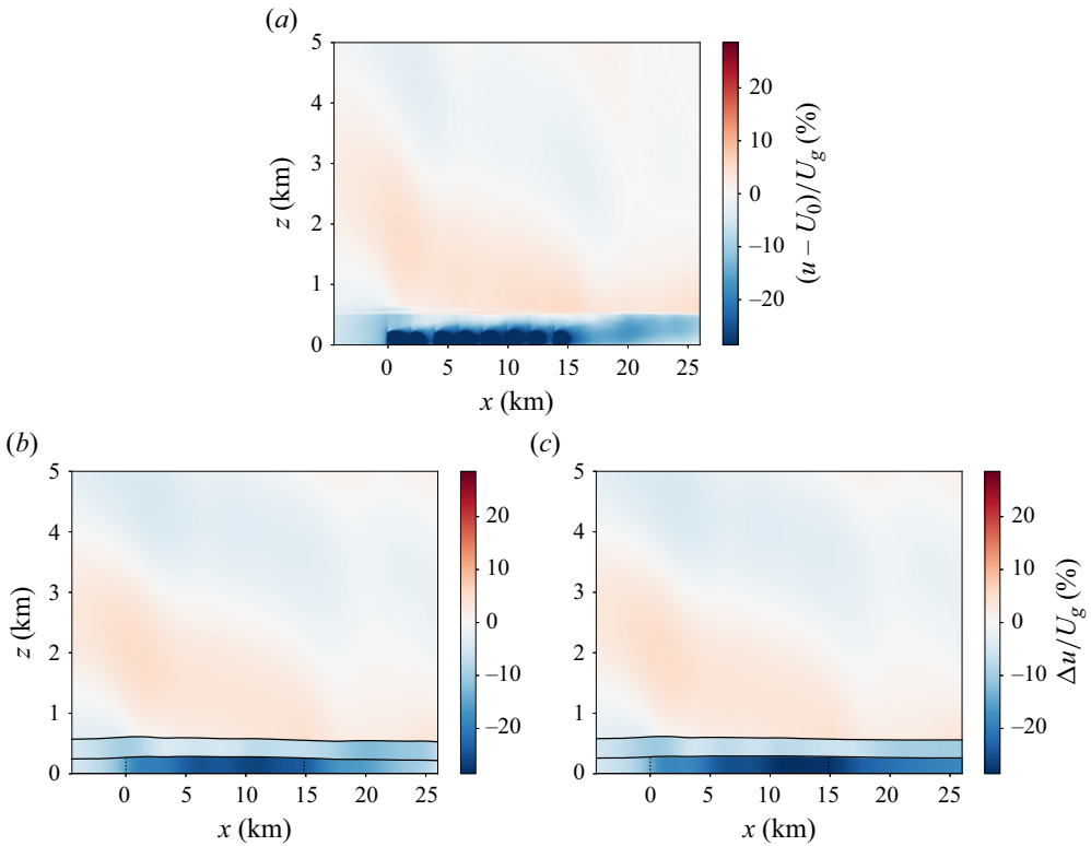
Figure 9. (a) Cross-section through the centre of the farm of the velocity perturbation for the case H500- \Delta\theta 5 - \Gamma 4 , as found by LES. Cross-section through the centre of the farm of the velocity perturbation for the APM state based on the LES results (b) and as found by the APM (c) for the case H500- \Delta\theta 5 - \Gamma 4 . The solid black lines denote the pliant surfaces separating the APM layers while the dashed lines show the wind farm region. The flow above the capping inversion is found using linear gravity wave theory.
