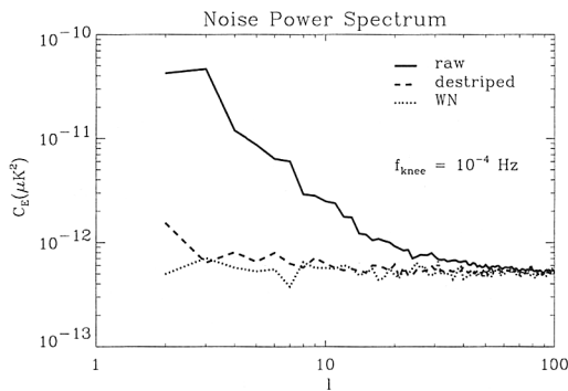
Figure 1. Angular power spectra (E mode) of noise maps obtained from simulations of the SPOrt experiment. The solid and dashed lines represent the power spectra obtained for f_{\text{knee}} = 10^{-4} Hz, before and after destriping, respectively. For comparison, the dotted line shows the power spectrum without 1/f noise ( f_{\text{knee}} = 0 ).
